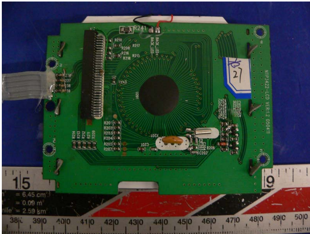
Base - Solder View 4
