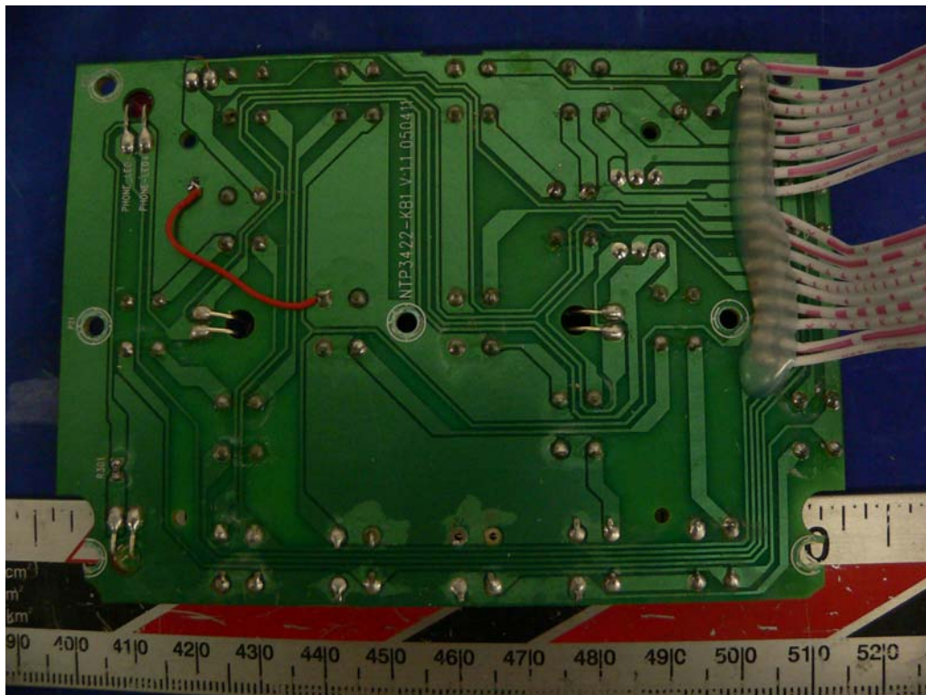
Base - Solder View 5
