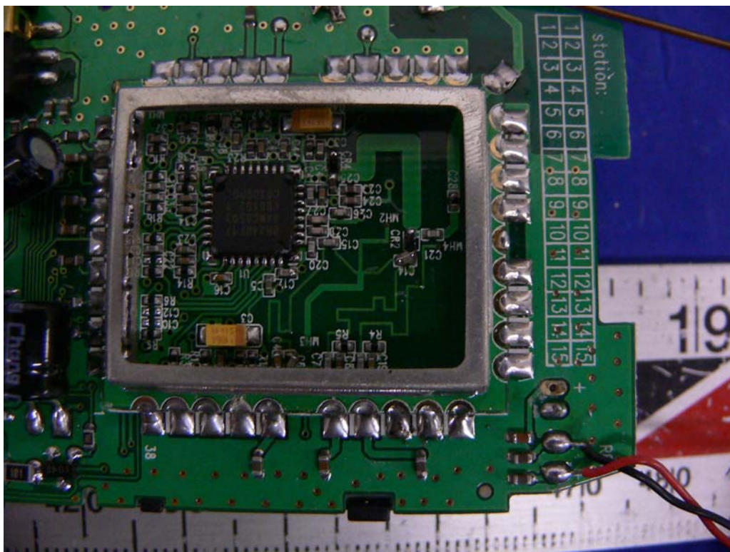
Handset – TX Cover Off View
