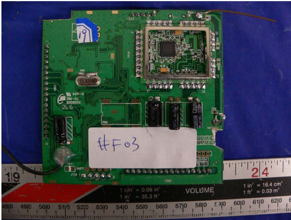
Base – TX Cover Off View
