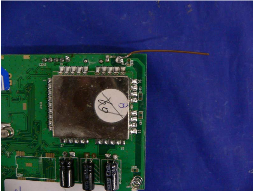
Base – TX Antenna Close View
