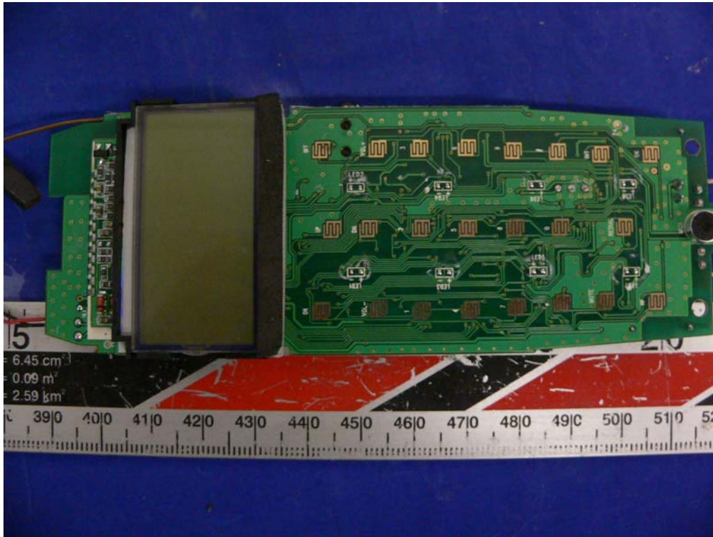
Handset – Solder View
