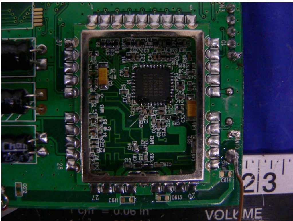
Base – TX Cover Off Close View
