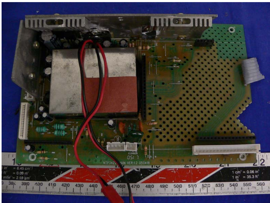
Base - Component View 3
