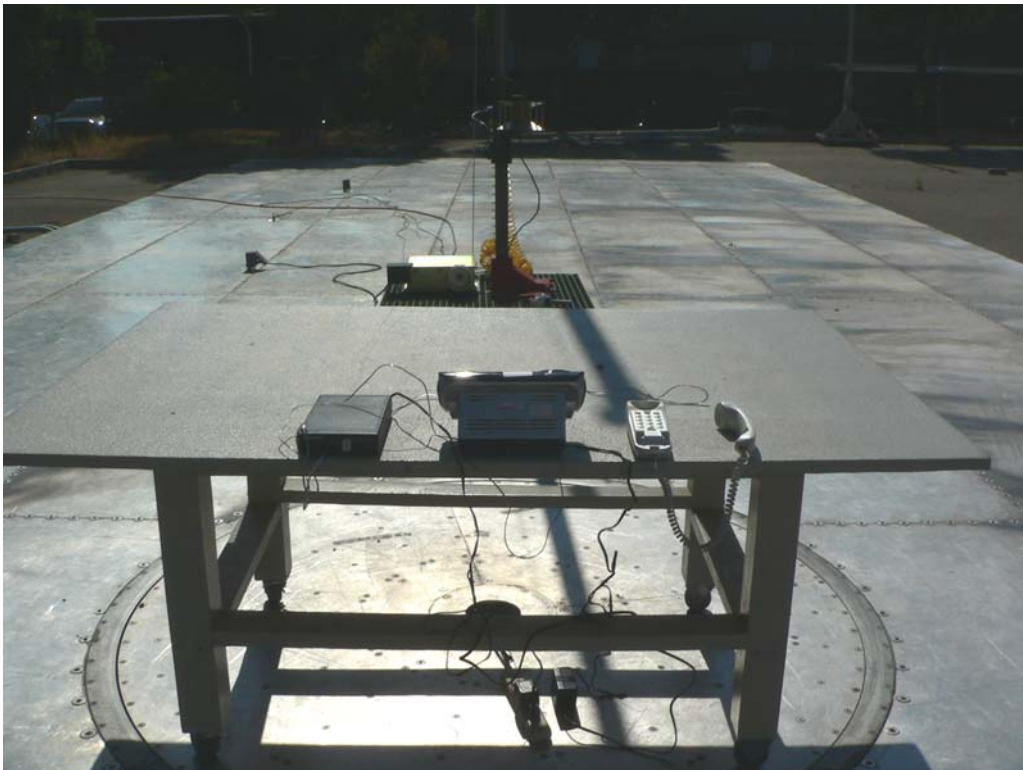
Radiated Emission - Rear View for Base
