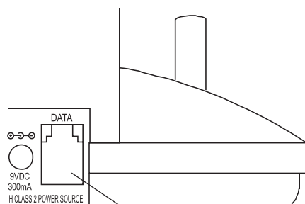
Data Jack
