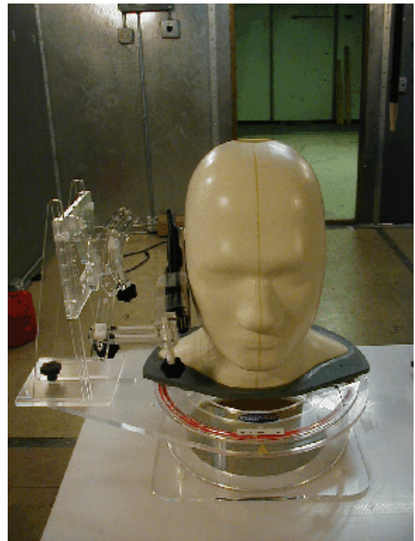
Figure S12. Configuration #12 - Cheek ( 0^{\circ} ) position, left side, GPS Out, 1200 mAH Battery
