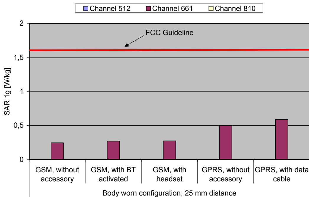
Fig. 9: The measured SAR values in body-worn configuration for the Benefon TPG 80EG for GPRS 1900 (Class 10) in comparison to the FCC exposure limit.
