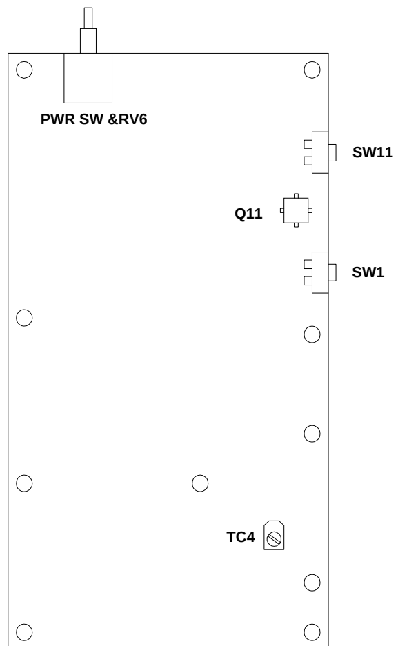
BOTTOM VIEW
