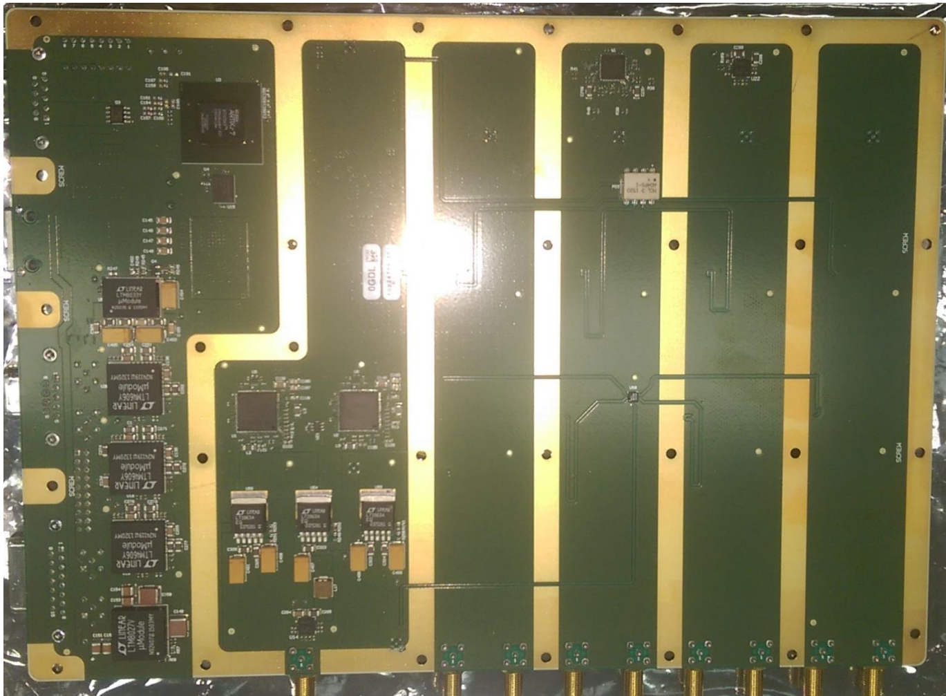
Digital Radar Board: Bottom View
