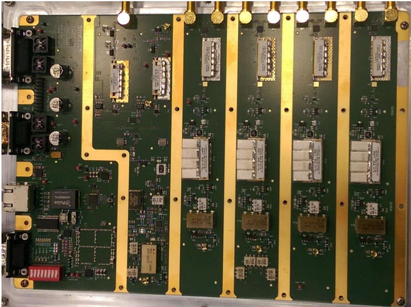
Digital Radar Board: Top View
