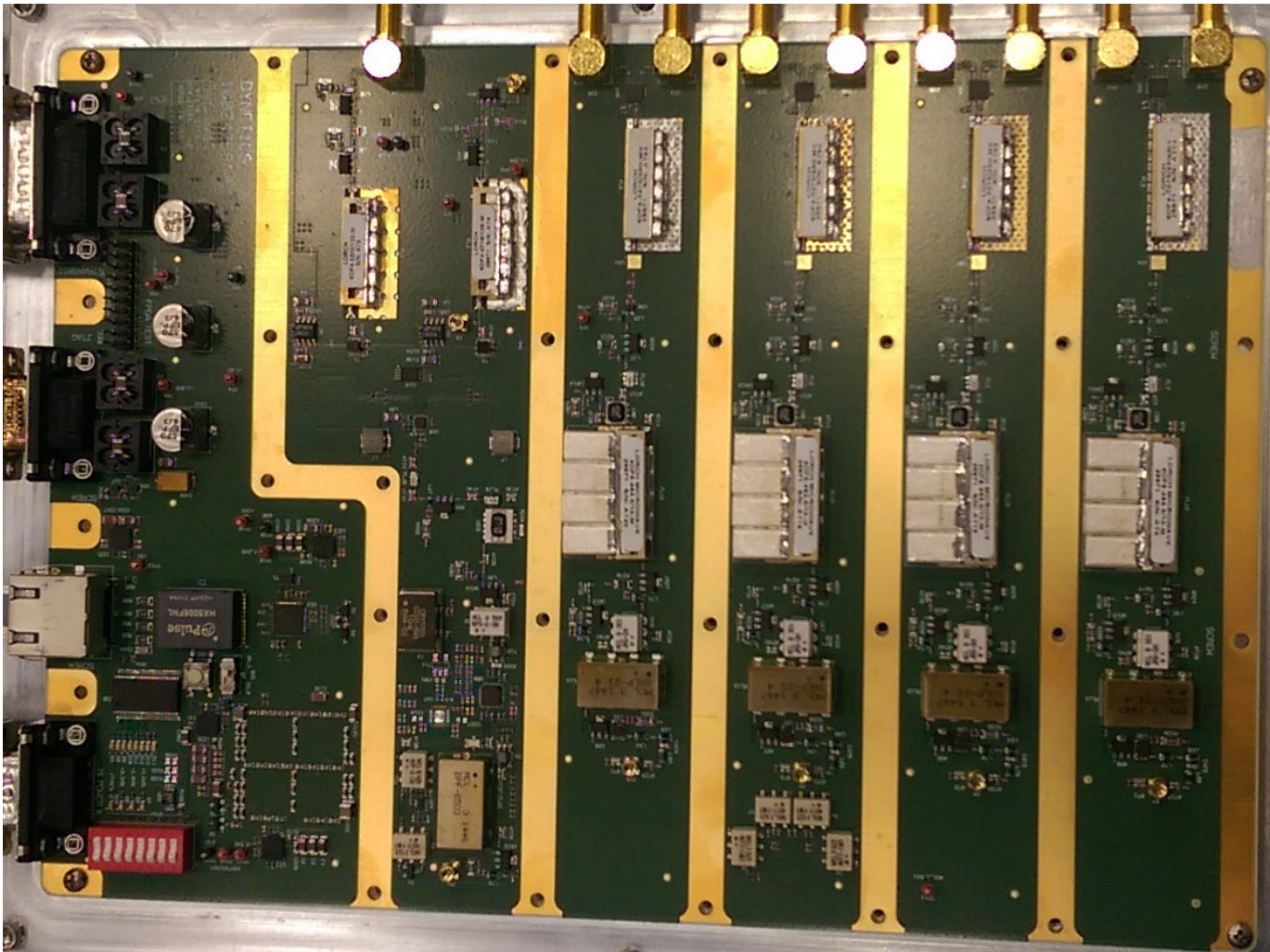
Digital Radar Board Outside of EMI Enclosure: Top View
