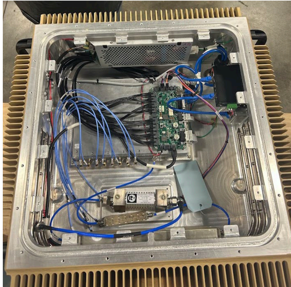
Central Enclosure
