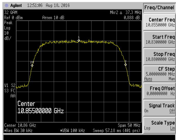
32 QAM @ 10855 MHz
