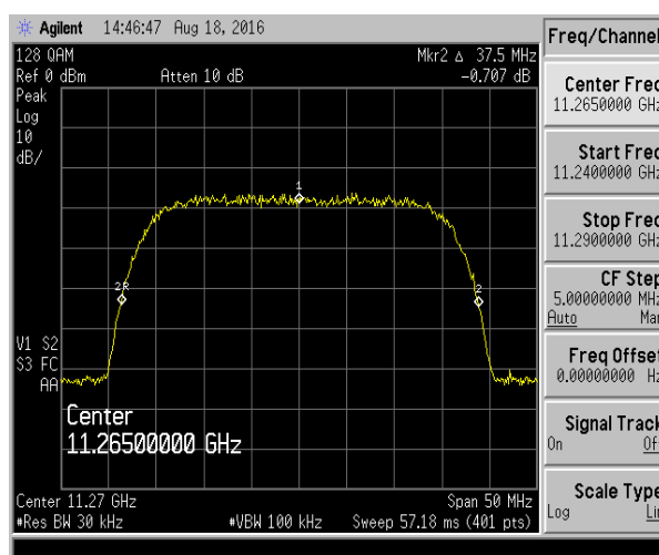
128 QAM @ 11265 MHz
