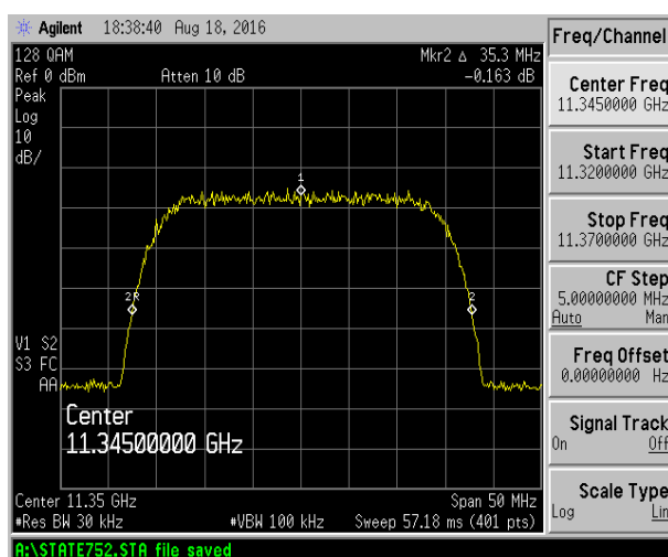
128 QAM @ 11345 MHz
