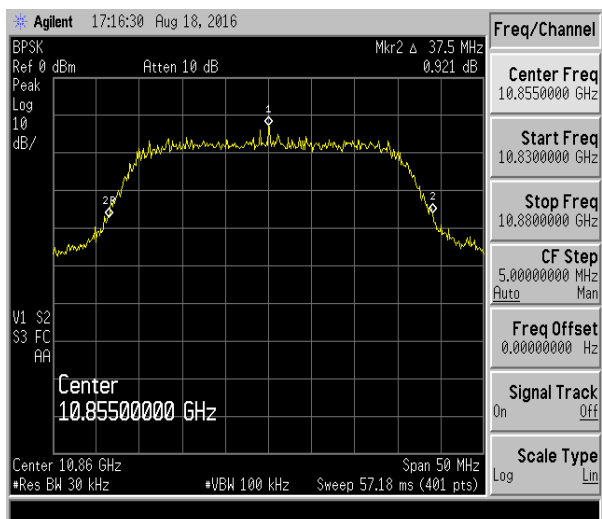
BPSK @ 10855 MHz
