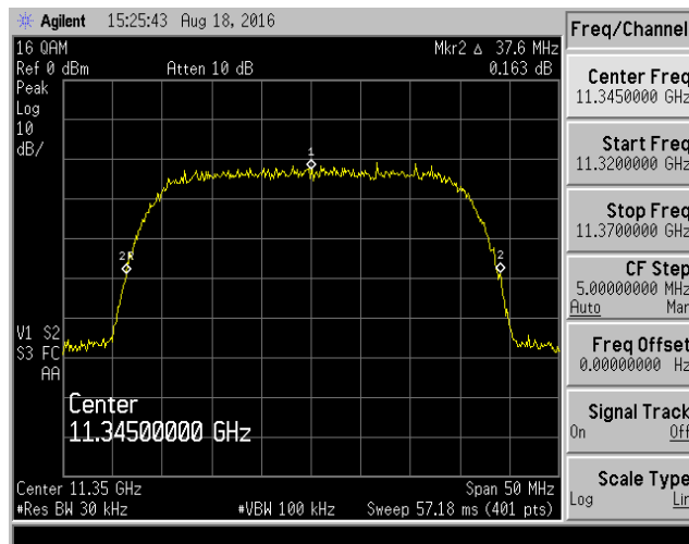
16 QAM @ 11345 MHz
