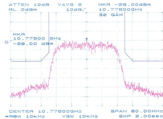
32 QAM @ 10775 MHz
