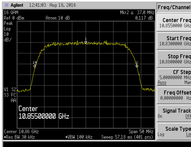
16 QAM @ 10855 MHz
