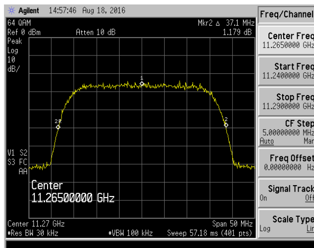
64 QAM @ 11265 MHz
