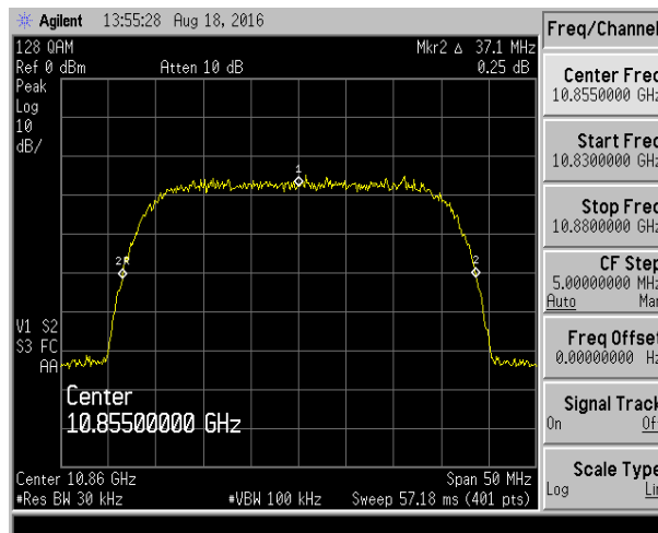
128 QAM @ 10855 MHz
