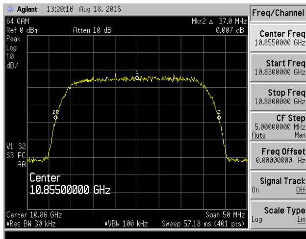
64 QAM @ 10855 MHz
