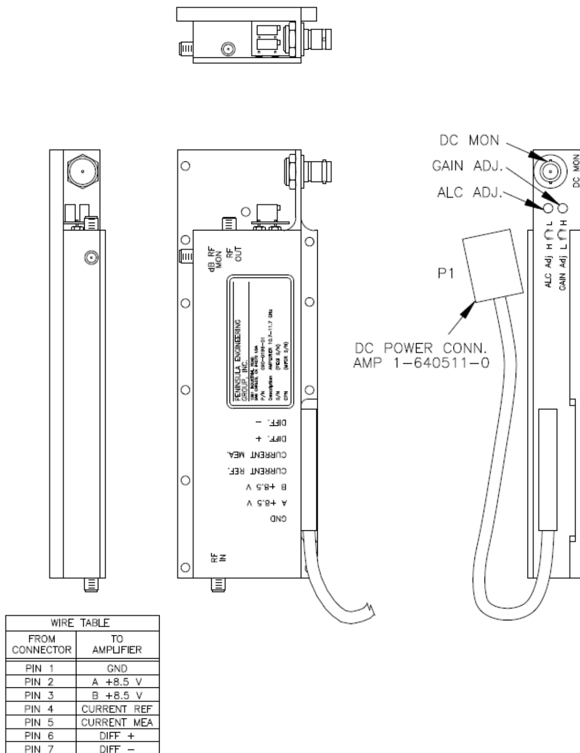
Figure 7 Linear Power Amplifier, Typical Outline
