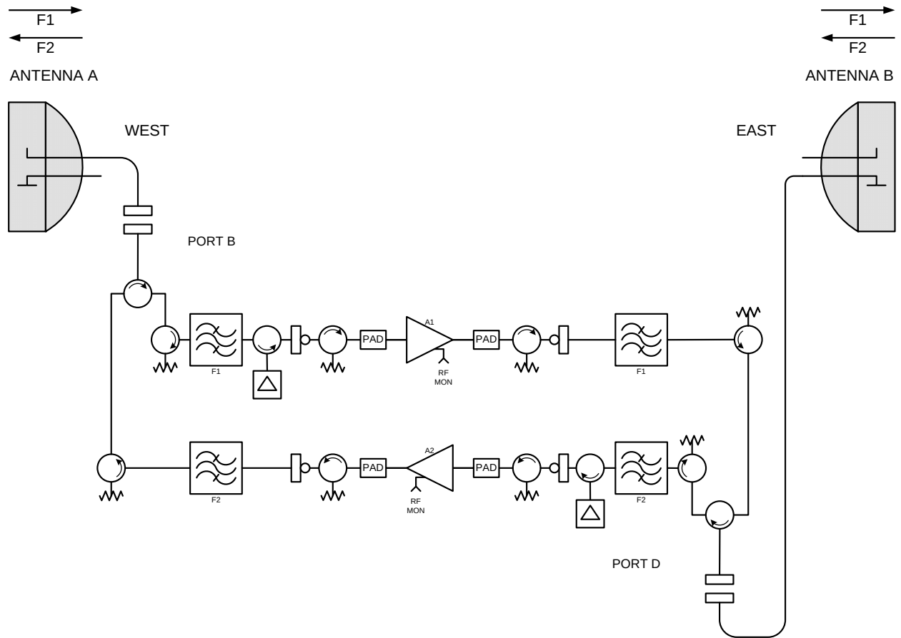
Figure 13 RF-11000E-051, 1+0 Delay Equalized
