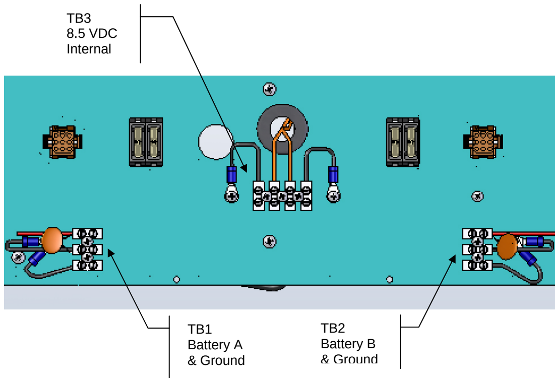
Figure 34 Wiring and Ground Connections, Main Repeater Panel
