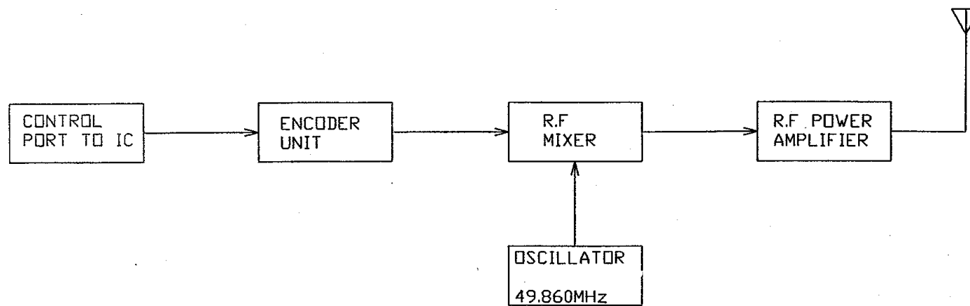
FUNCTION BLOCK DIAGRAM OF 49MHz TRANSMITTER
