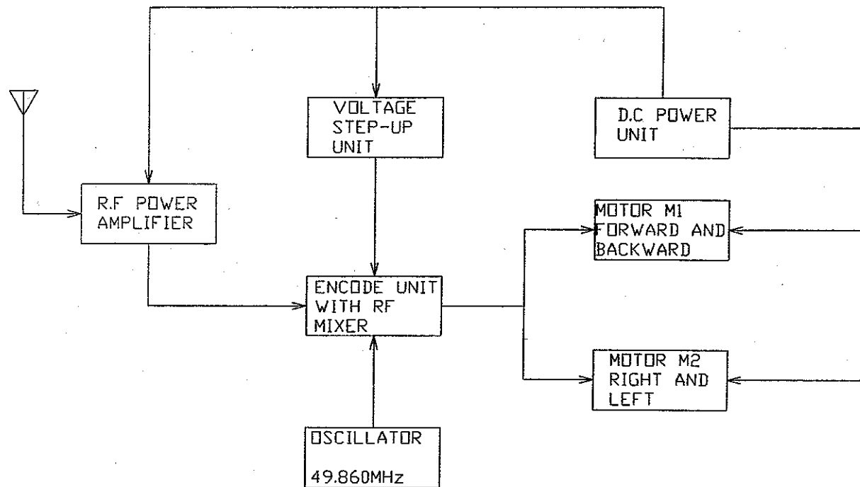
FUNCTIONAL BLOCK DIAGRAM OF 49MHz RECEIVER
