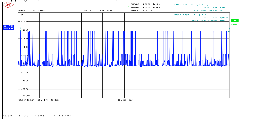
Hopping on, number of transmissions, channel 38
