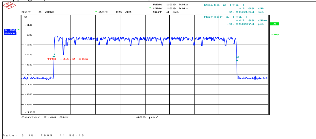
Hopping on, duration of one transmission, channel 38
