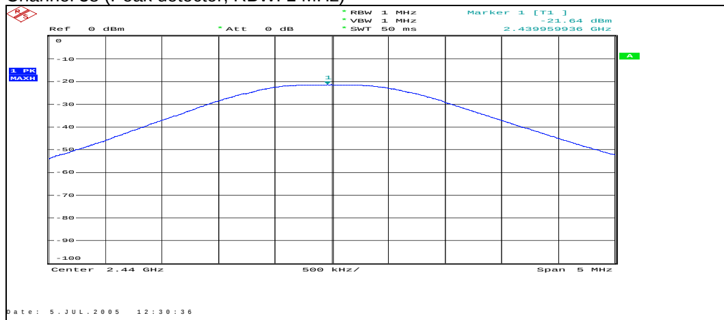
Channel 38 (Peak detector, RBW: 1 MHz)
