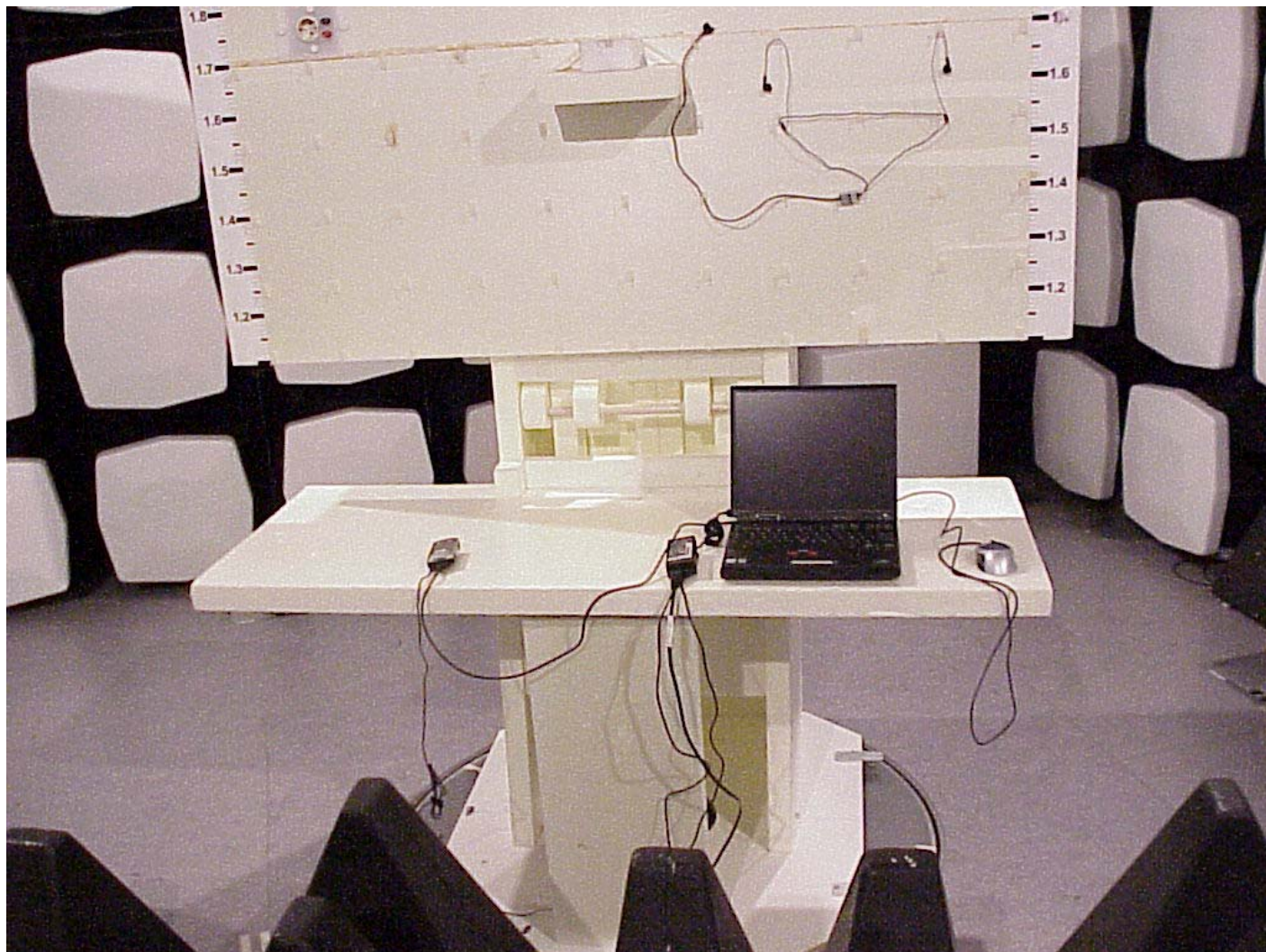
Part 15B Radiated Emission
