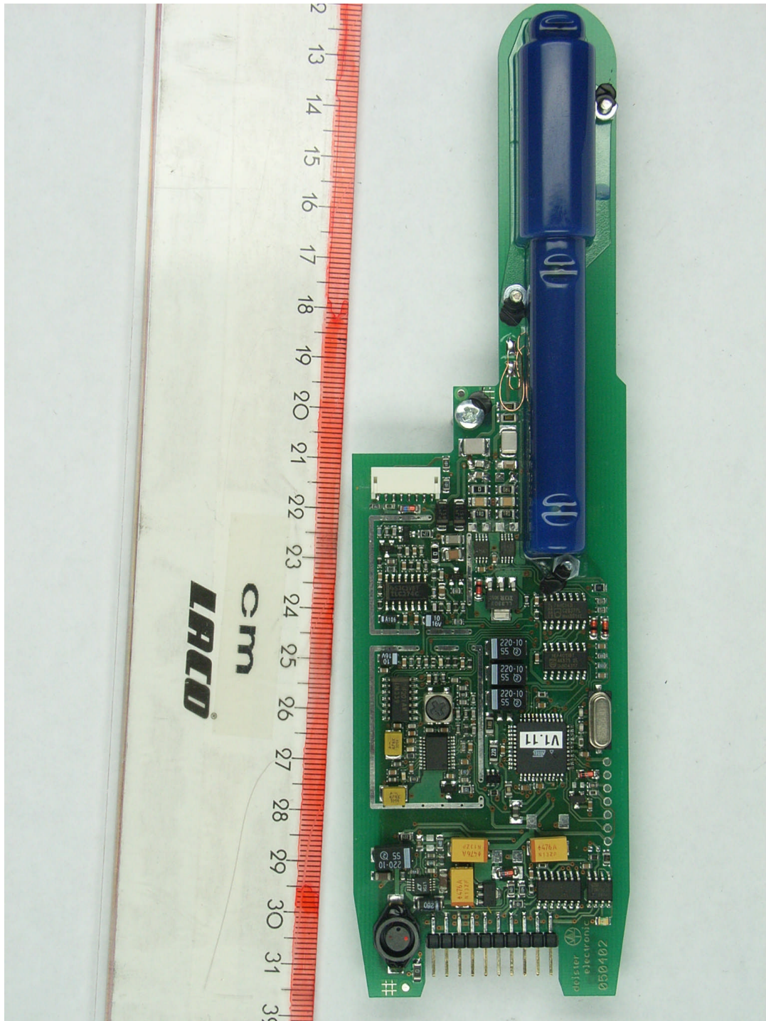
52017_2a.jpg AIR200 PCB, top view
