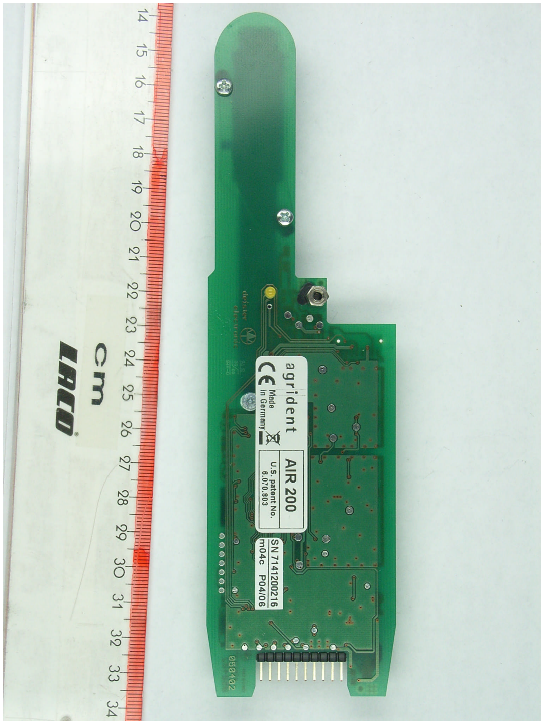
52017_2b.jpg AIR200 PCB, bottom view
