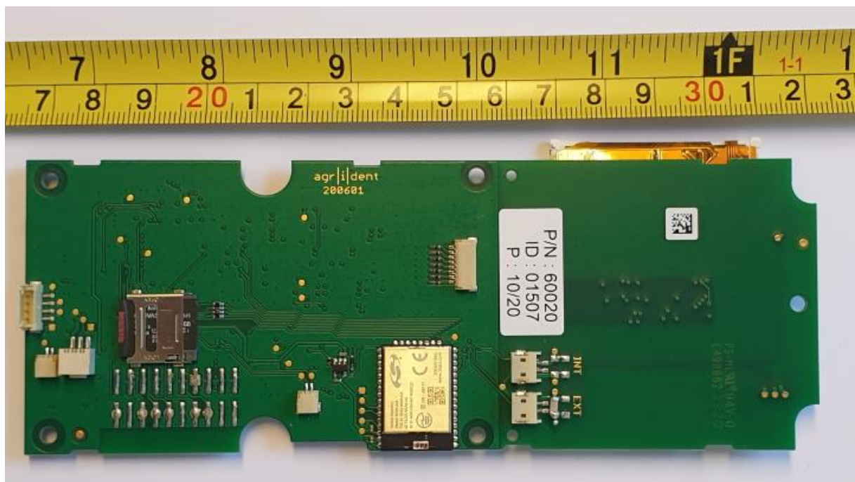
Main PCB Bottom View (for APR250, APR600 and APR650)
