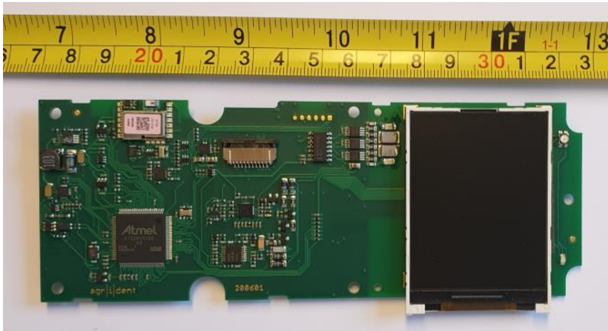
Main PCB Top View (for APR250, APR600 and APR650)
