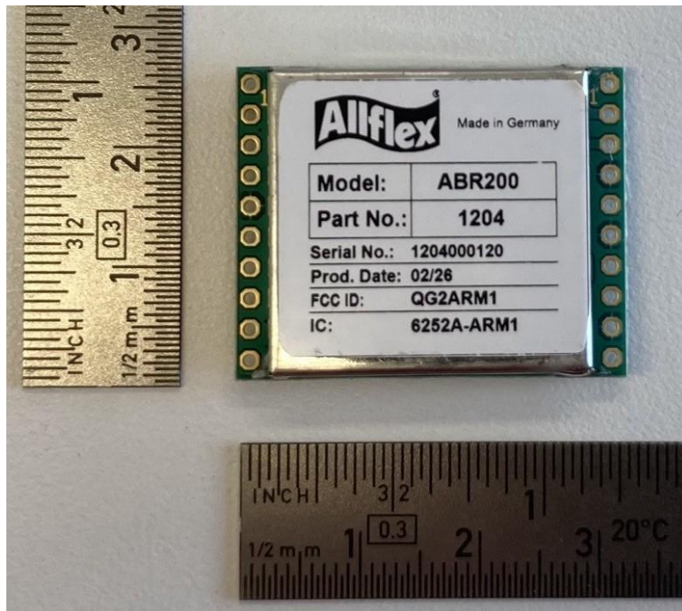
ABR200 top (with shielding)
