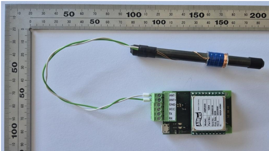
ABR200 on adapter board with 100mm ferrite antenna
