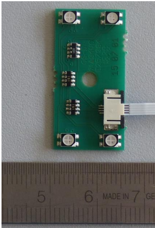
LED-board top view:
