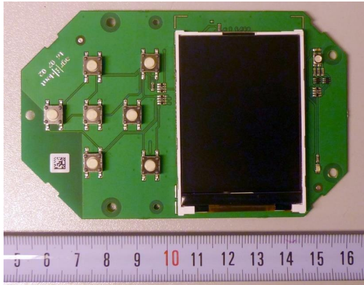
Displayboard top view:
