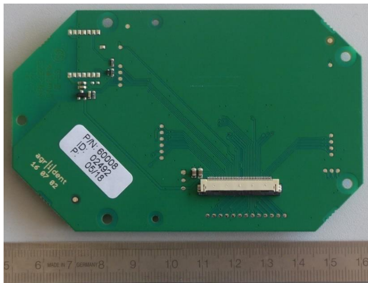
Displayboard without WLAN bottom view:
