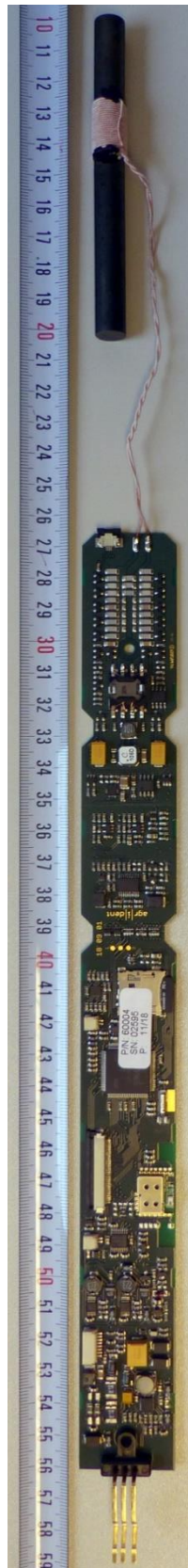
Mainboard with antenna top view:
