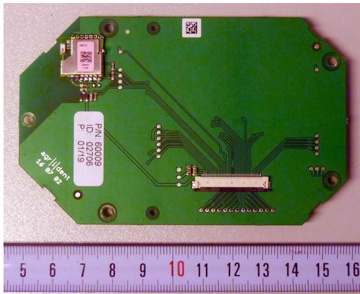
Displayboard with WLAN bottom view:
