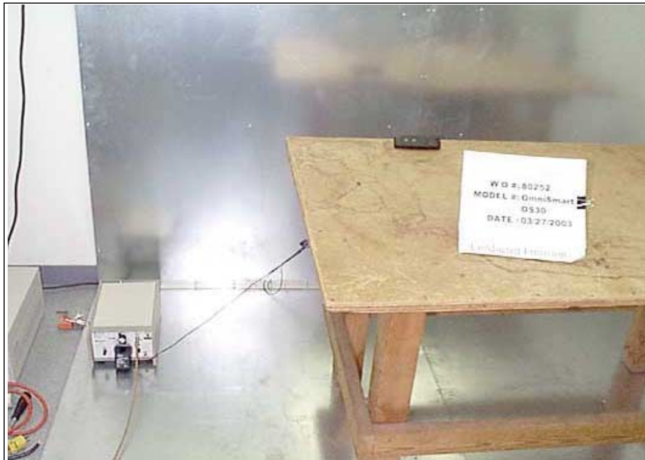
15.207 Front View
