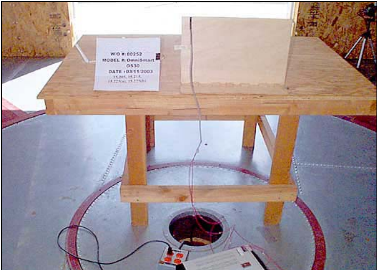
15.209, 15.215 & 15.225 Back View
