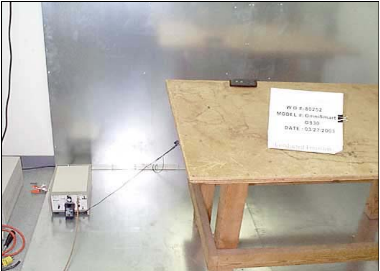
15.207 Front View
