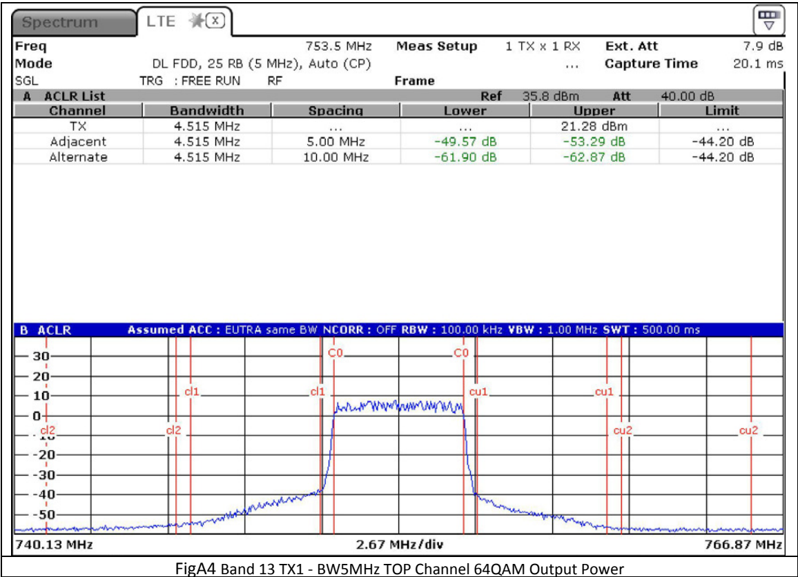
FigA4 Band 13 TX1 - BW5MHz TOP Channel 64QAM Output Power
