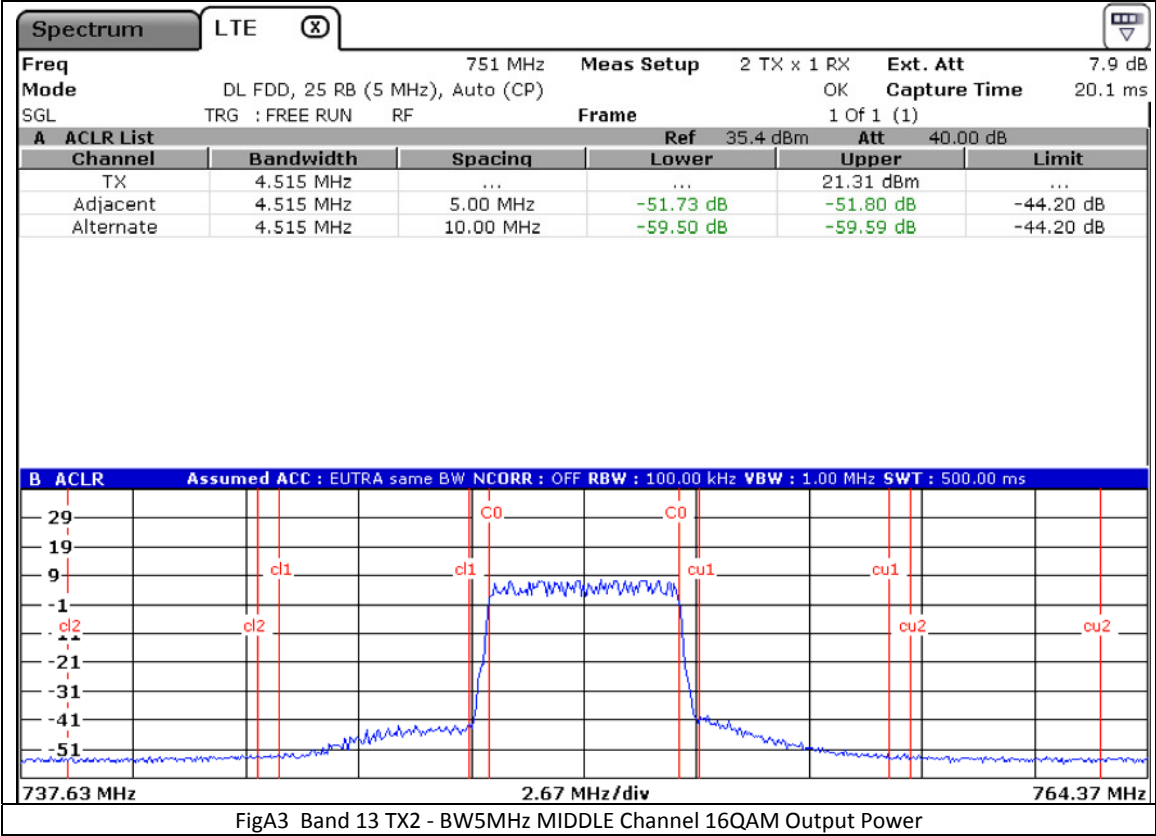
FigA3 Band 13 TX2 - BW5MHz MIDDLE Channel 16QAM Output Power
