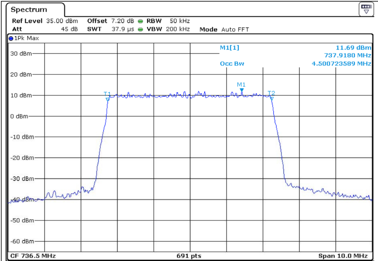
Fig B7 Band 17 TX1 - BW5MHz BOTTOM Channel QPSK Occupied Bandwidth
