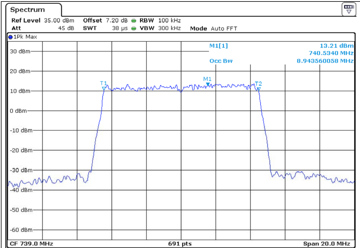
Fig B8 Band 17 TX1 - BW10MHz BOTTOM Channel 16QAM Occupied Bandwidth
