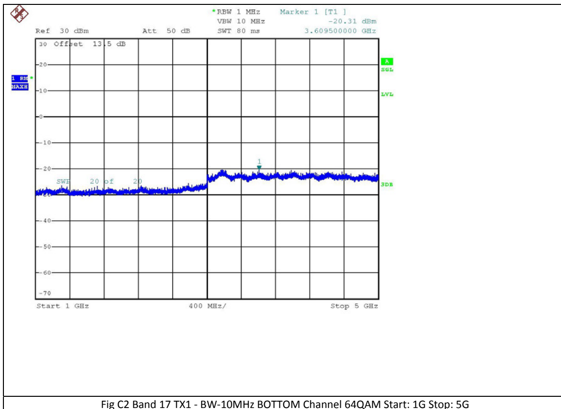
Fig C2 Band 17 TX1 - BW-10MHz BOTTOM Channel 64QAM Start: 1G Stop: 5G
