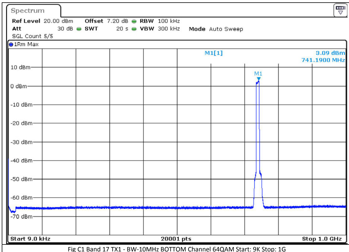
Fig C1 Band 17 TX1 - BW-10MHz BOTTOM Channel 64QAM Start: 9K Stop: 1G
