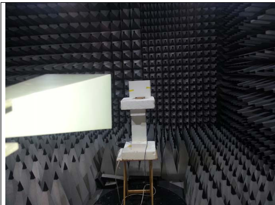
Fig 4 Test setup 18-22GHz Rad Emission
