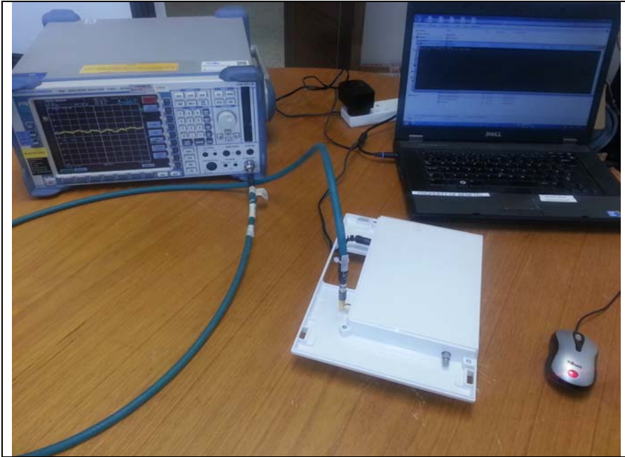
Fig 1 Test setup Conducted Emissions on Antenna port
