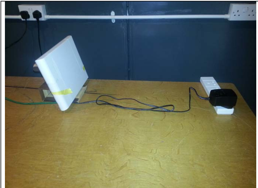
Fig 8 Test setup Conducted Emissions on the mains
