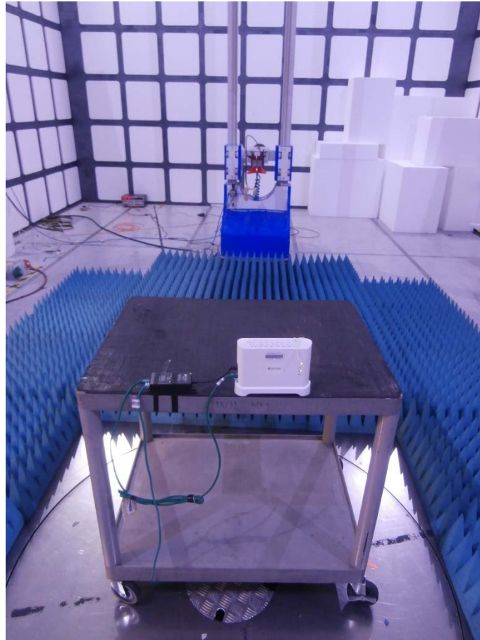
Radiated Emissions 1 GHz to 10 GHz using PoE
