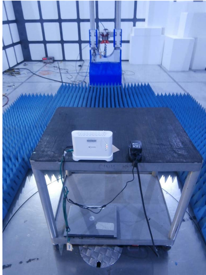
Radiated Emissions 1 GHz to 10 GHz using PSU
