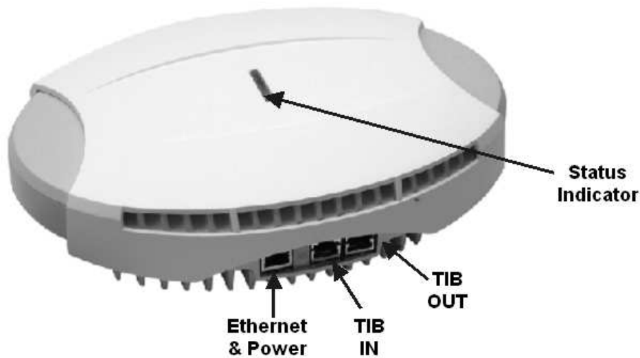
Figure 8 - nanoBTS Connections
