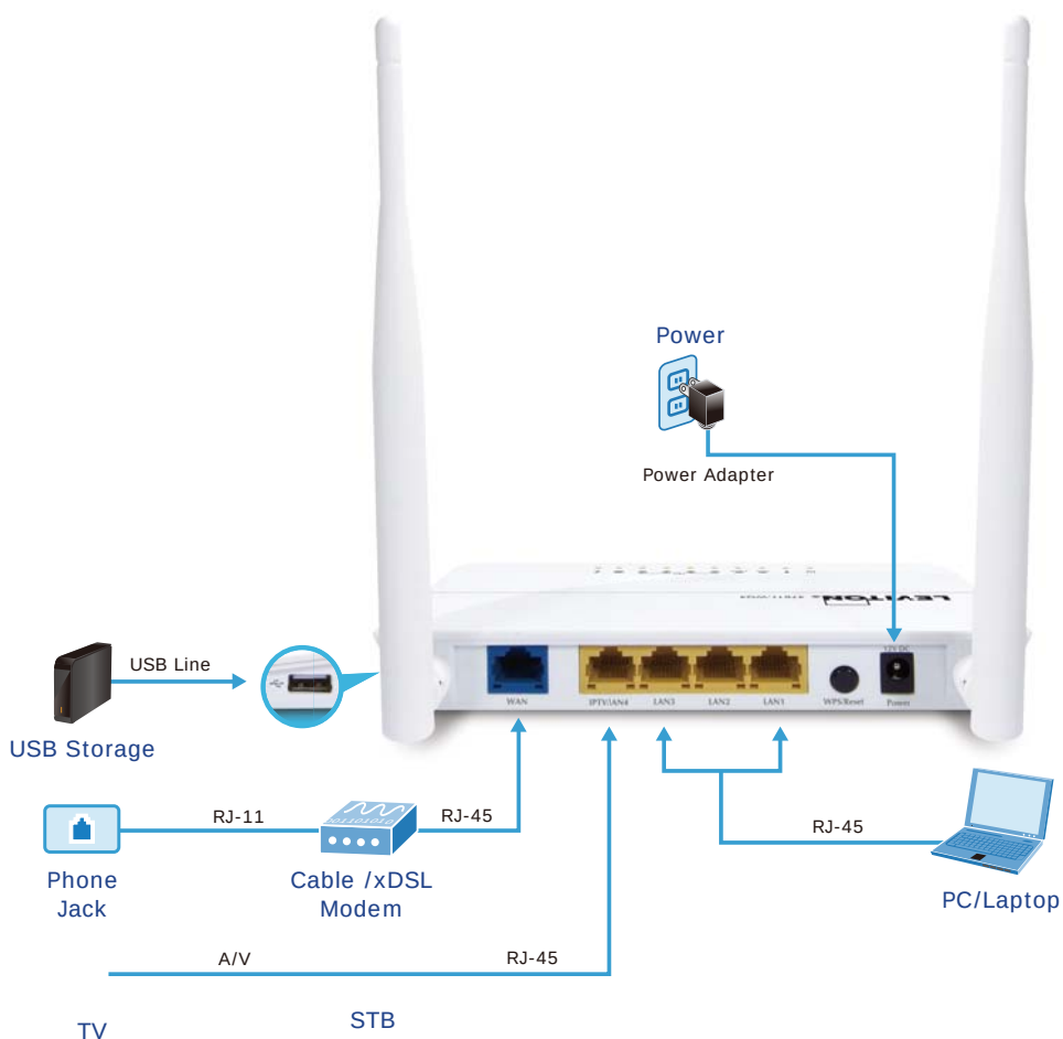
Figure 3-2 Hardware Installation-2
