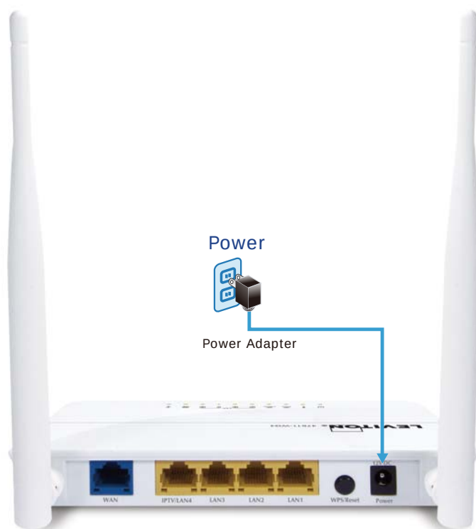
Figure 3-1 Hardware Installation-1
