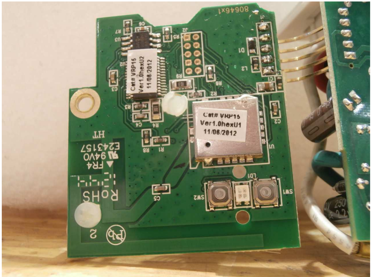
RF board top view
