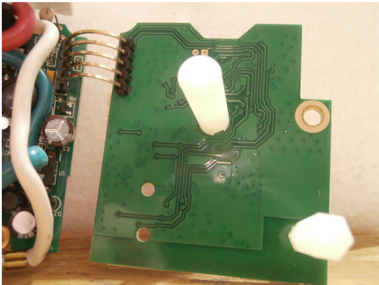
RF board bottom view
