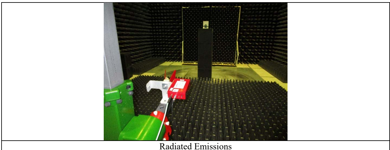
Radiated Emissions
