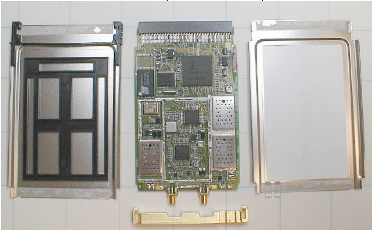
Disassembled (Some Shields Removed)
