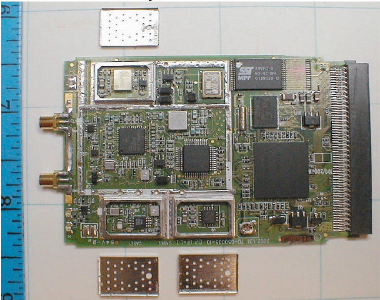
Top, All Shields Removed
