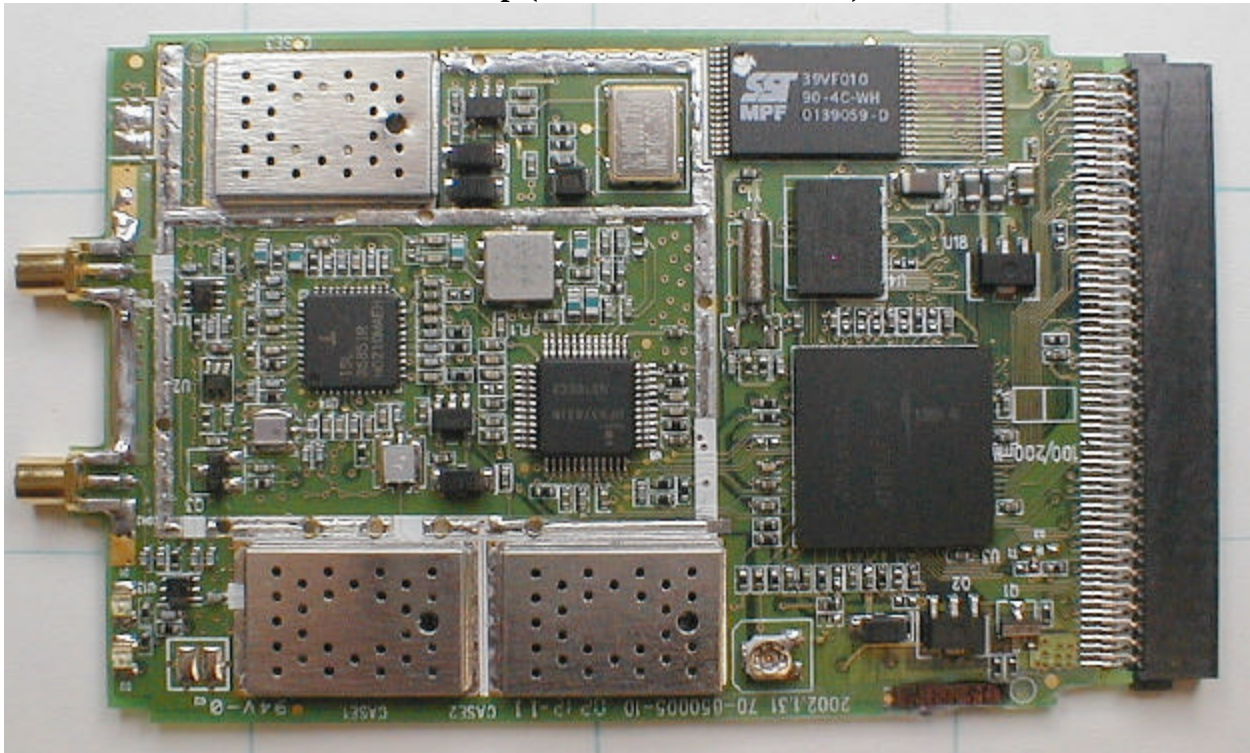
PCB Top (Some Shields Removed)
