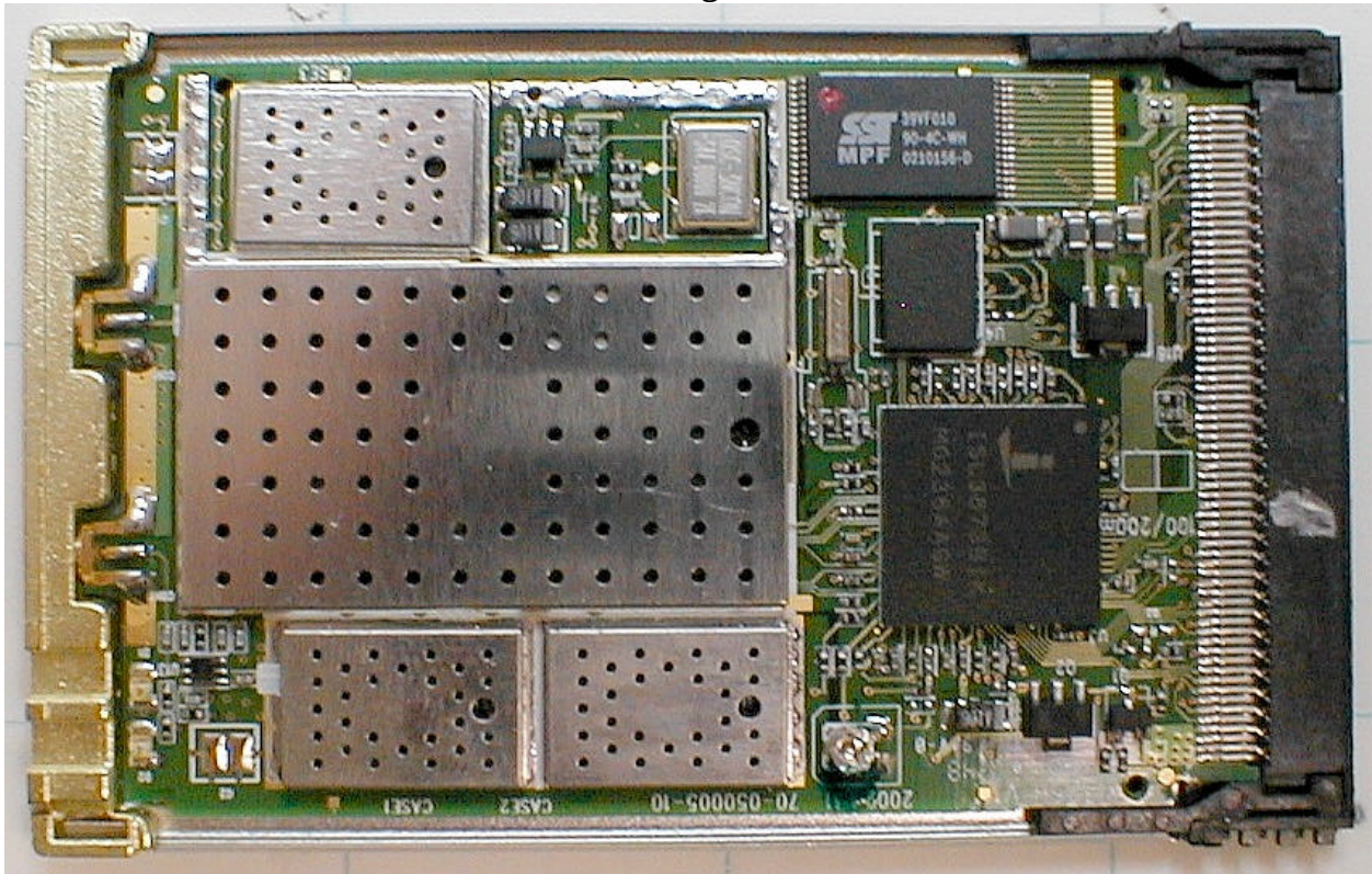
Covers Off, Showing Shields In Place
