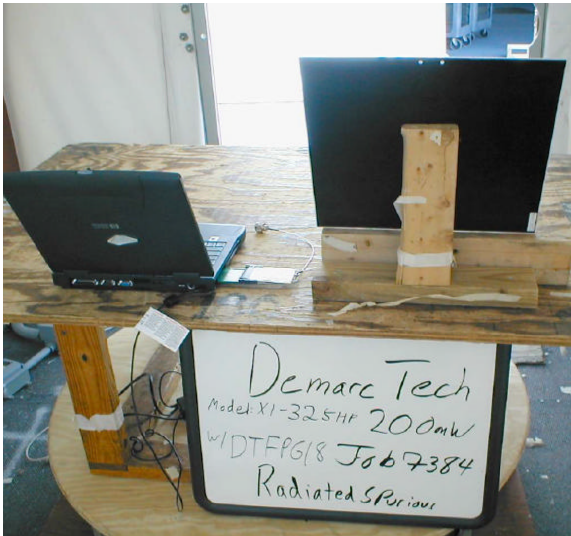
DTFPG18 Antenna, Back
