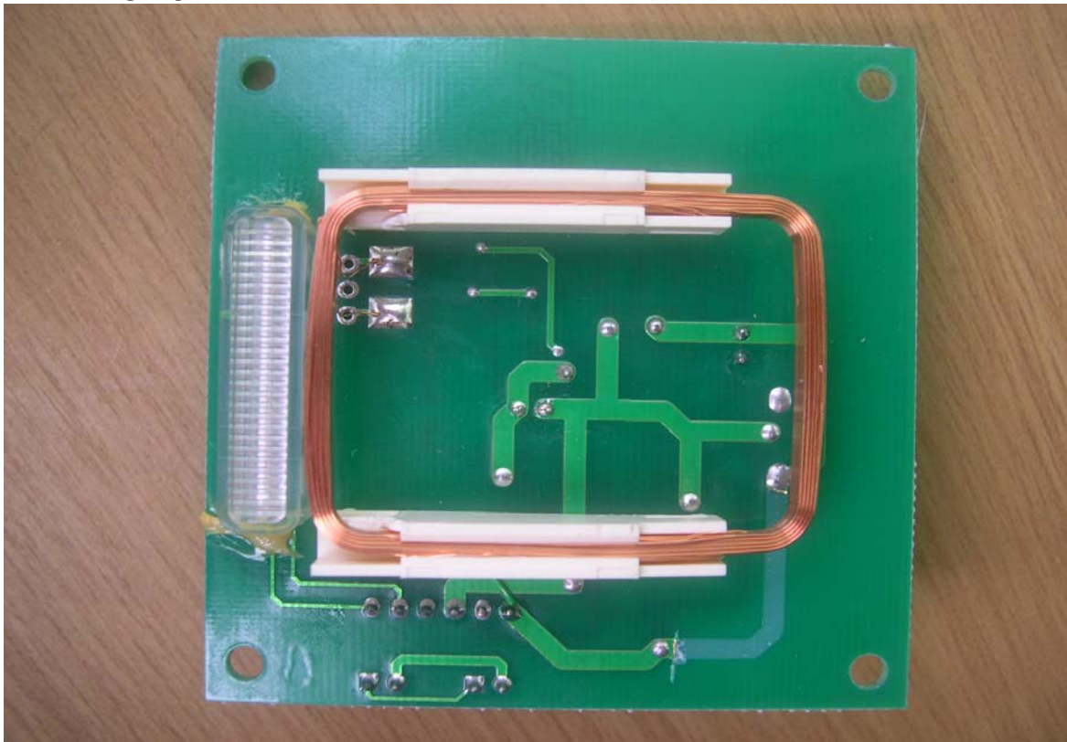
<Photograph 7: RF Card Transceiver Board Rear View >
