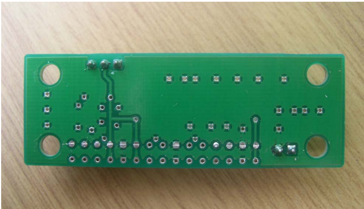
<Photograph 5: RF Control Receiver Board Rear View >
