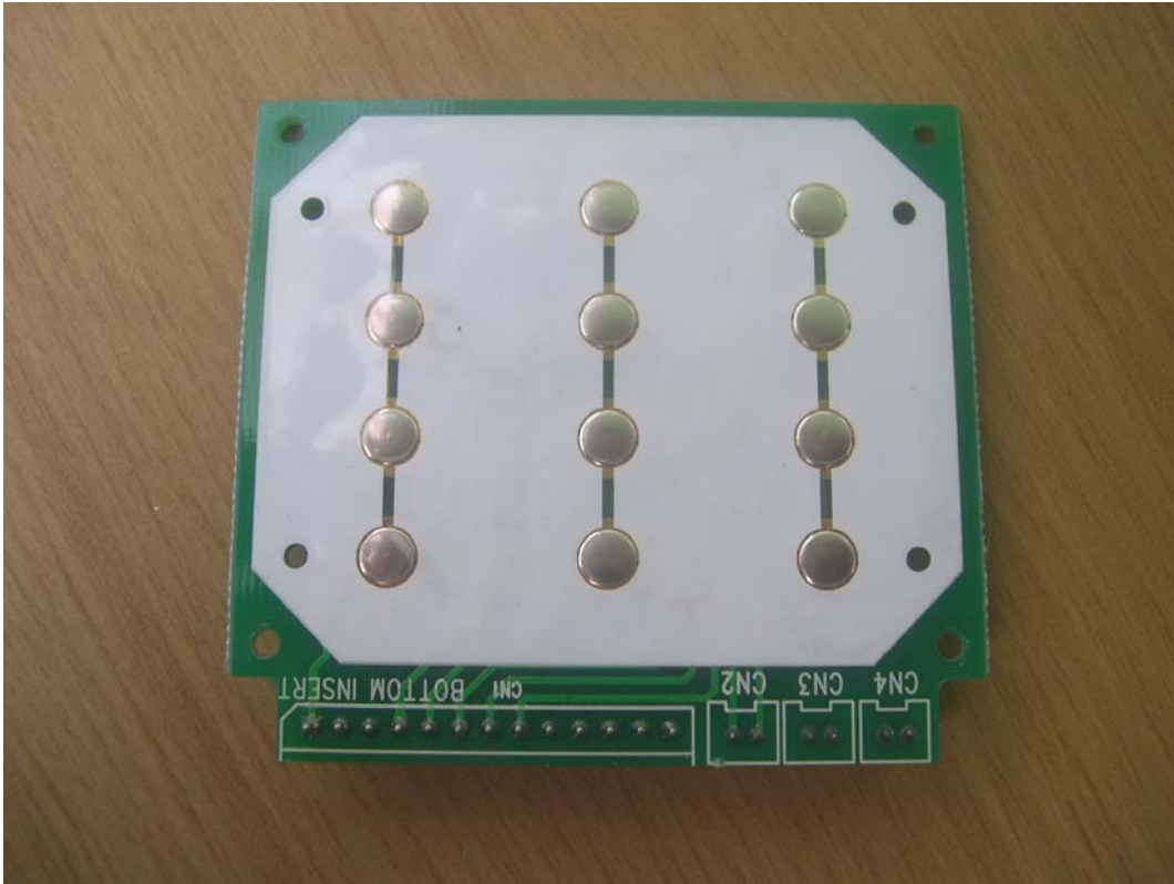
<Photograph 8: Keypad Board Rear View >
