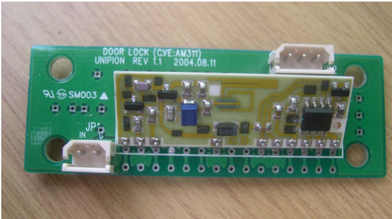
<Photograph 5: RF Control Receiver Board Rear View >
