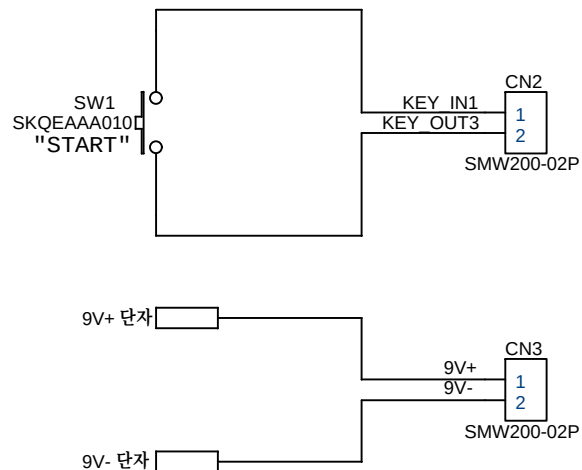
Front Board 3- BATT
