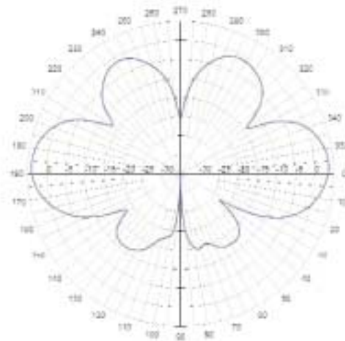
MFB24004 Elevation Cut
