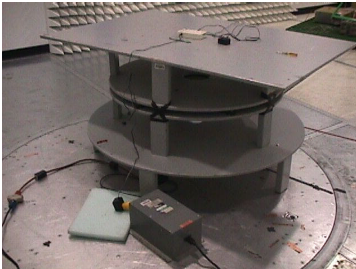
Conducted Emissions Test Configuration
