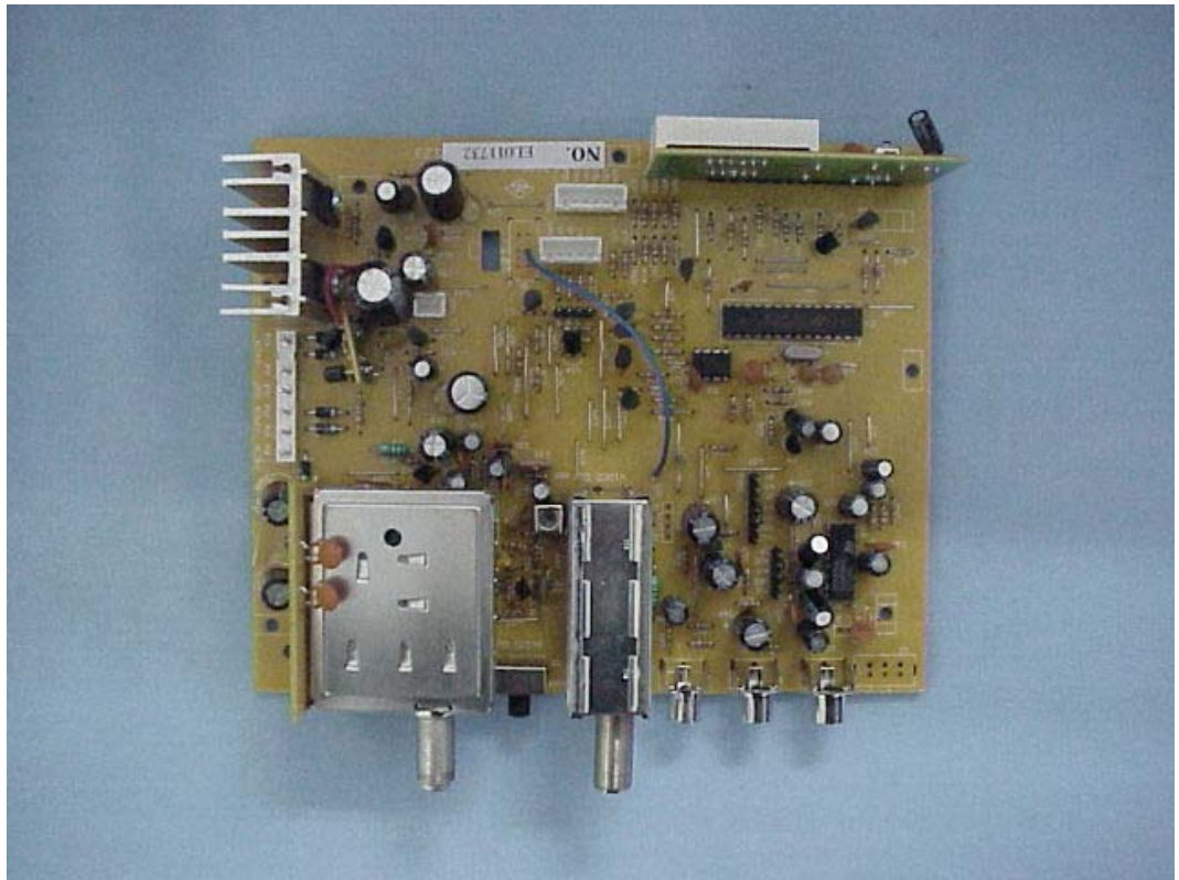
FIGURE 3 CATV CONVERTER (M/N: YT-F6688U) MAIN BOARD (COMPONENT SIDE)
