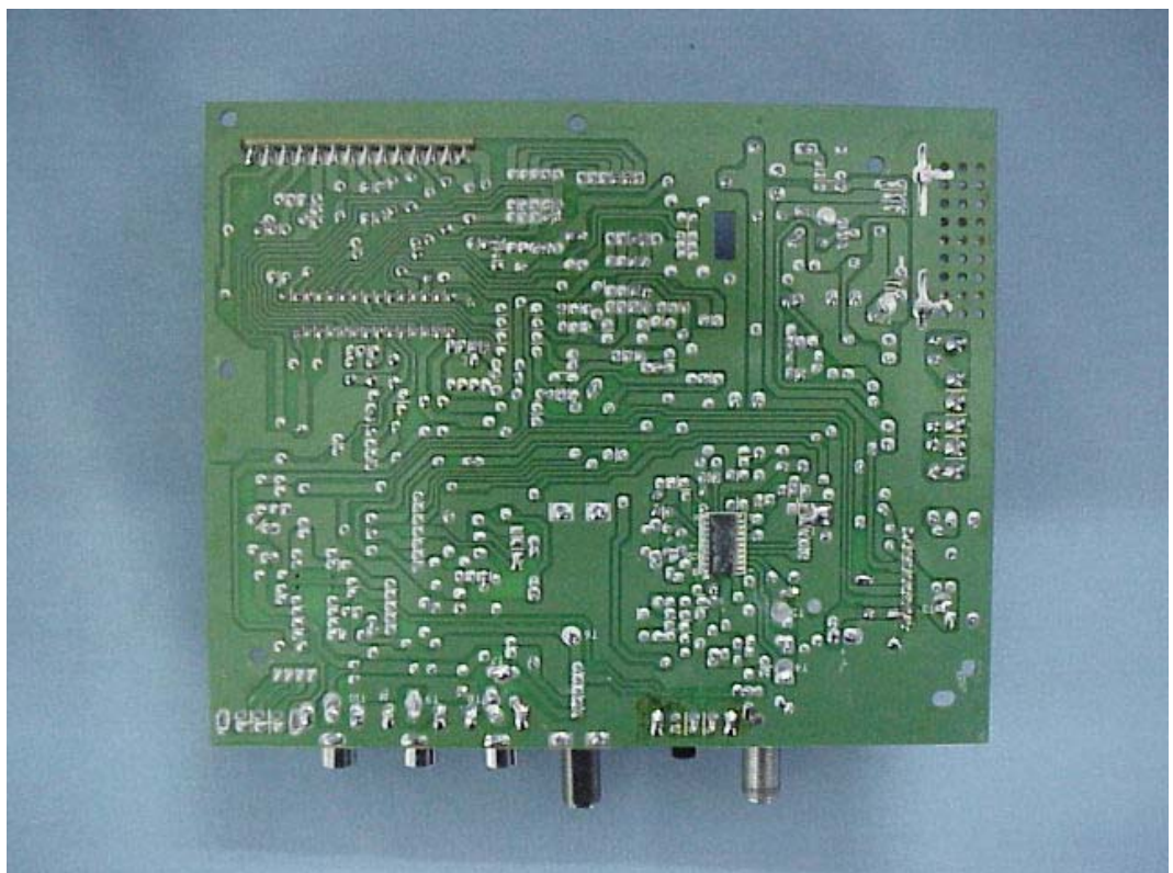
FIGURE 4 CATV CONVERTER (M/N: YT-F6688U) MAIN BOARD (SOLDERED SIDE)
