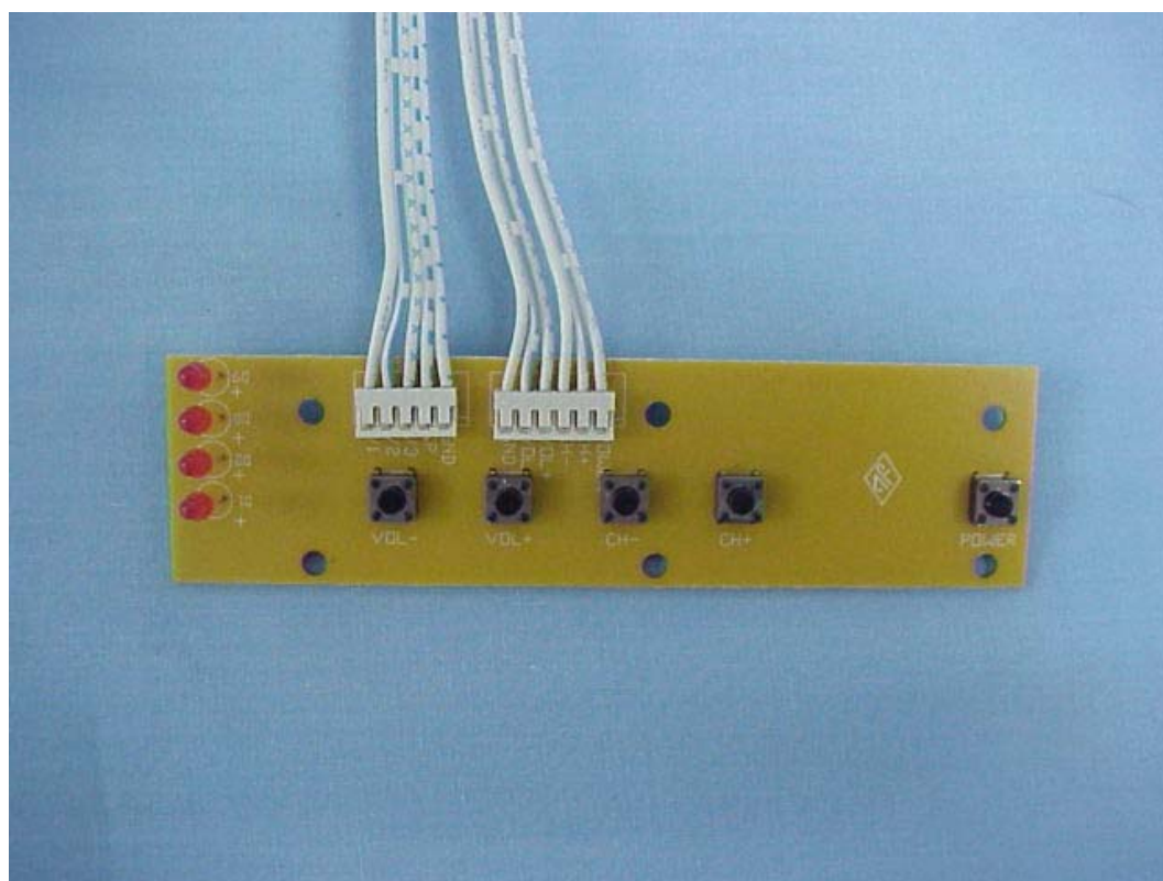
FIGURE 5 CATV CONVERTER (M/N: YT-F6688U) SWITCH BOARD (FRONT SIDE)
