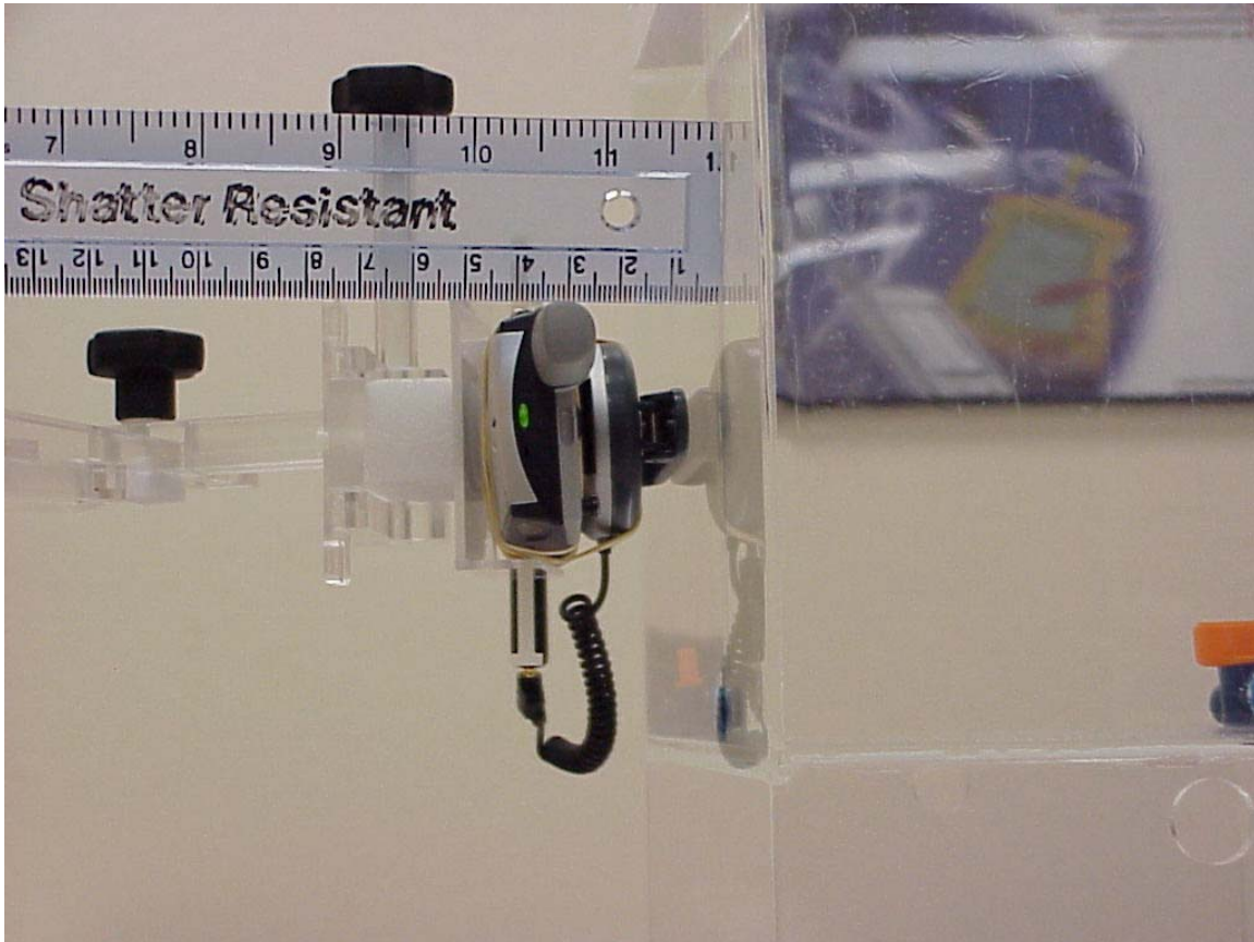
Photo 6: EUT belt clip configuration, EUT touching phantom distance.
