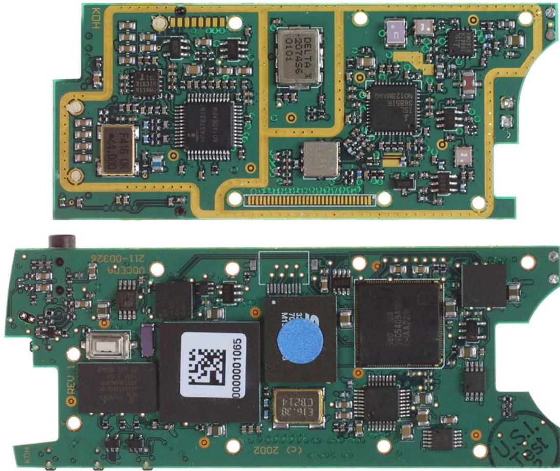
BOTTOM SIDES FOR BOTH BOARDS
