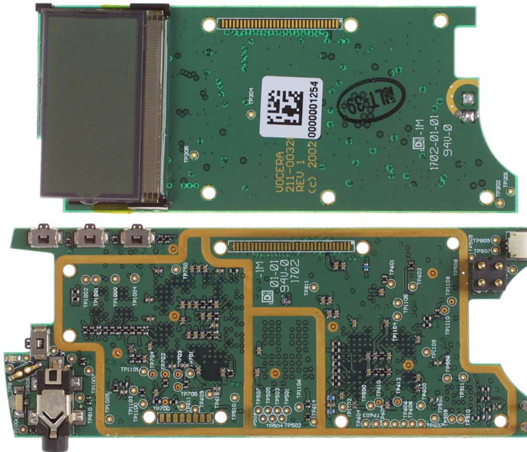
TOP SIDE OF BOTH BOARDS
