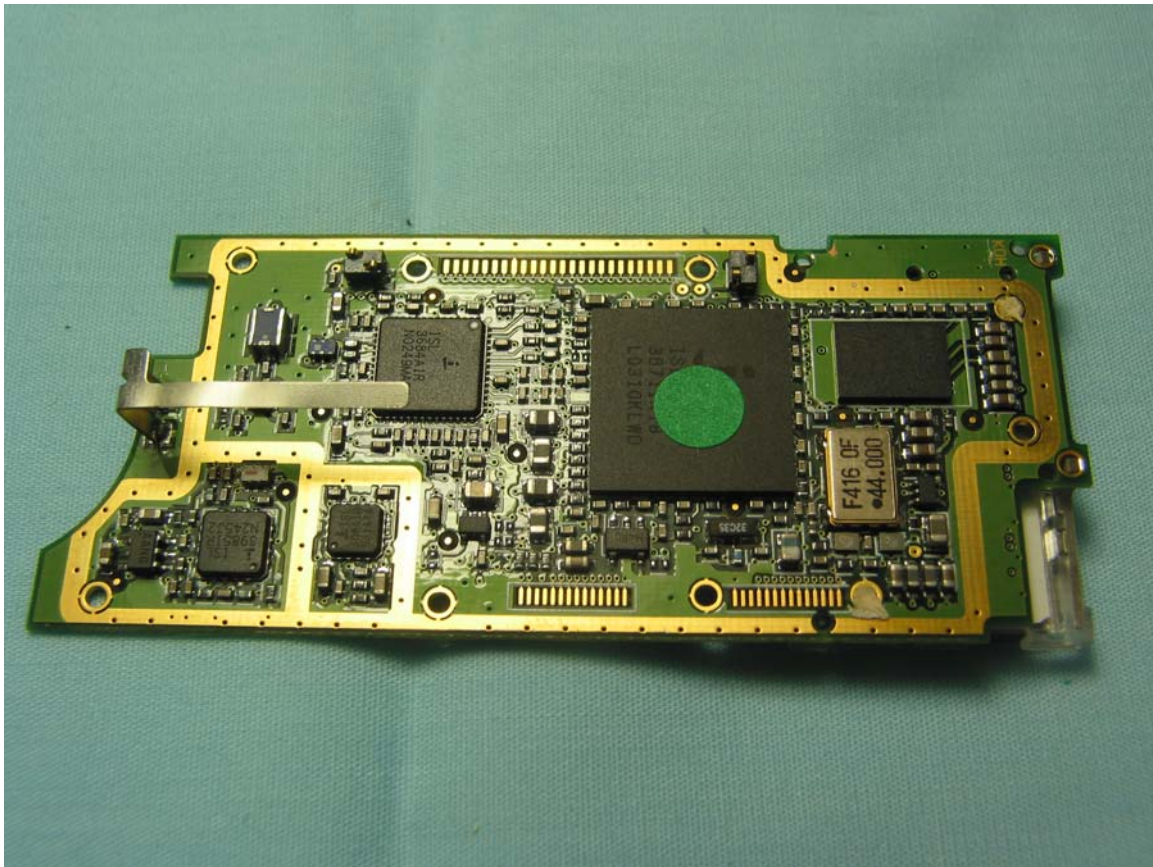
Display / RF board, RF side
