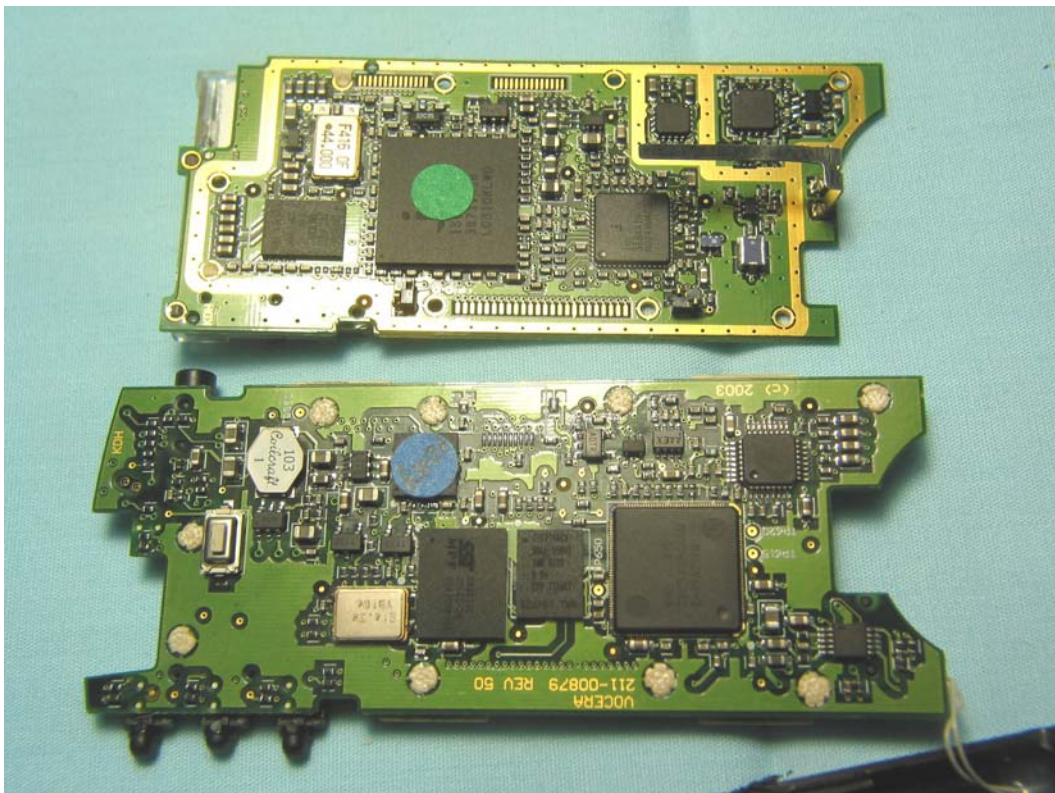
“Main” board & RF/Display board
