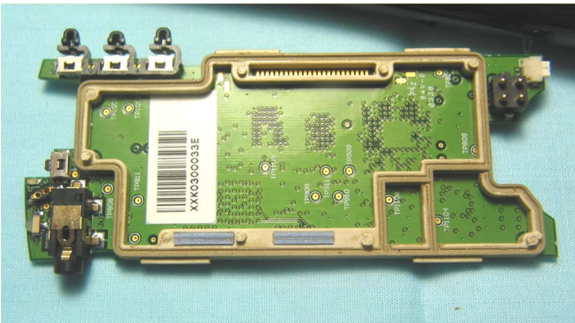
Main Board, rear view
