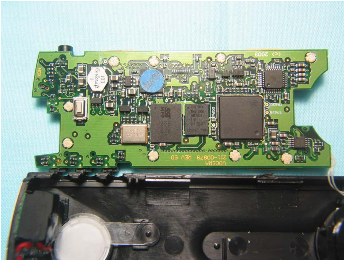
Main Board, Front View
