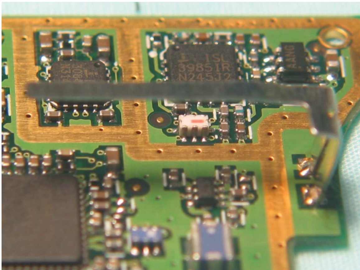
Close-up, antenna
