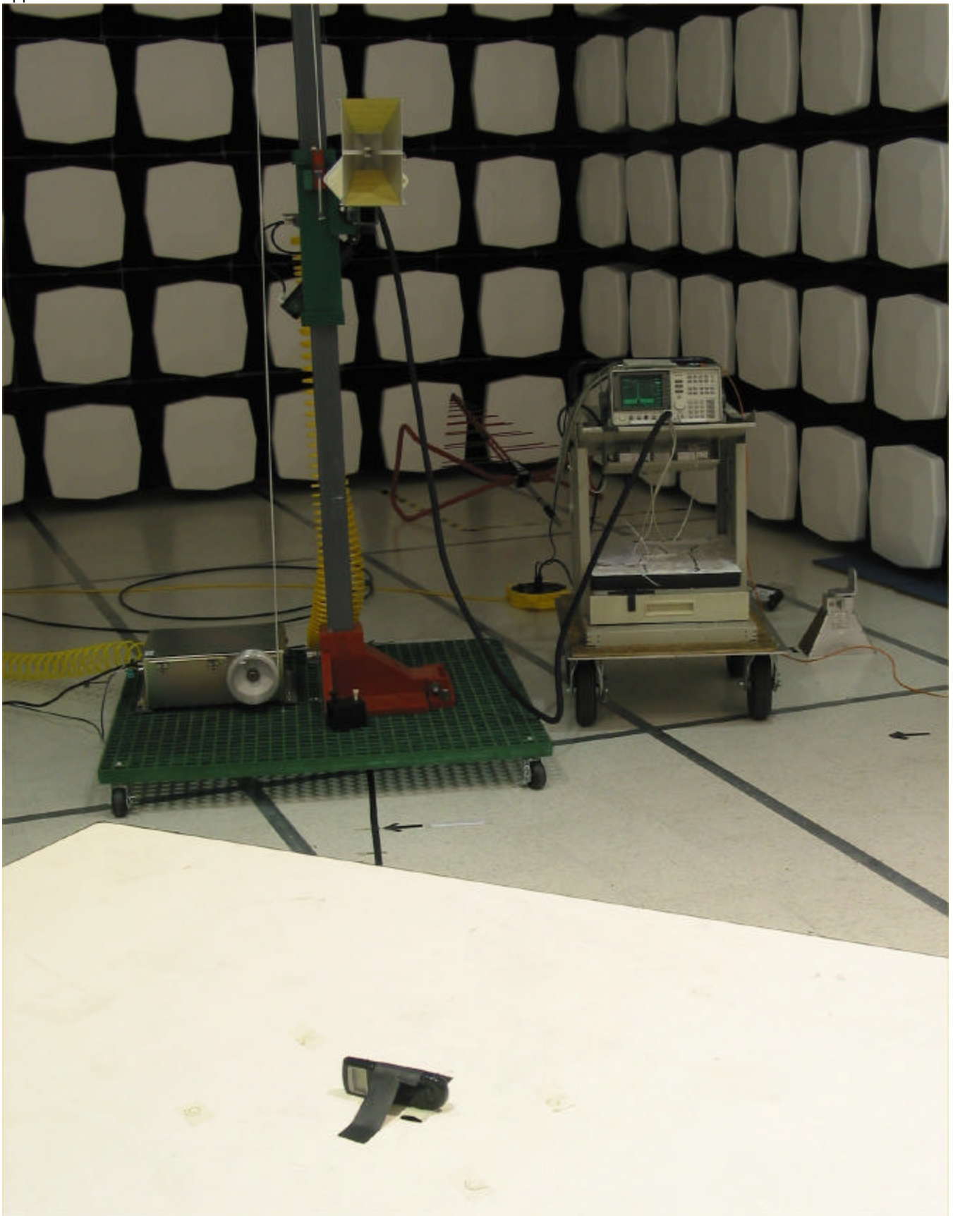
Radiated emissions, Anechoic Chamber
