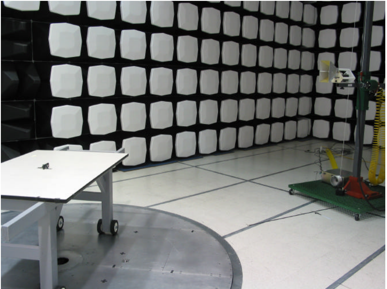
Radiated emissions, Anechoic Chamber
