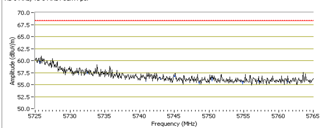
RB 1 MHz; VB 3 MHz Peak H-pol
