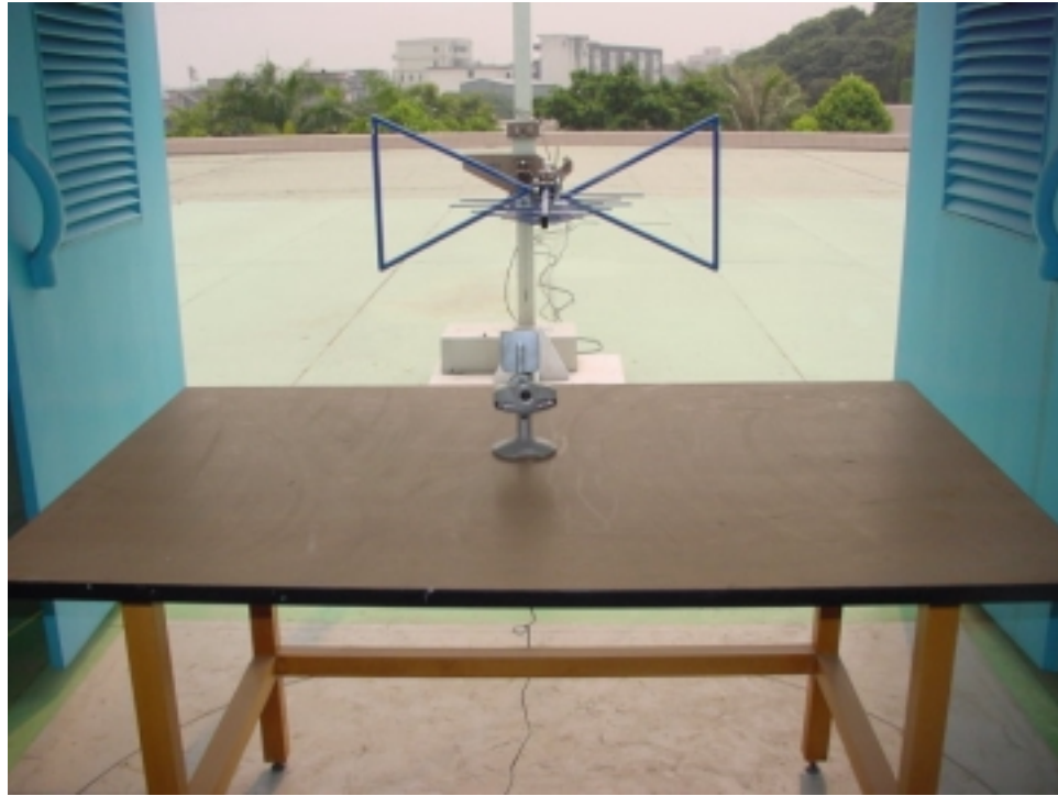
Photo7 Test Setup for Radiated Disturbance Test(Transmitter Front View)
