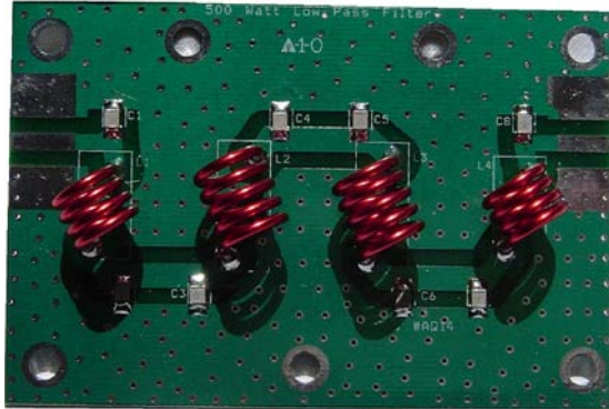
Lowpass Filter Construction (lid removed):
