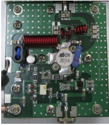
Power Amplifier Construction (lid removed):
