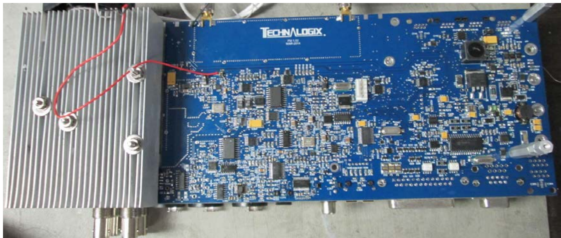
FM Exciter Construction (bottom):
