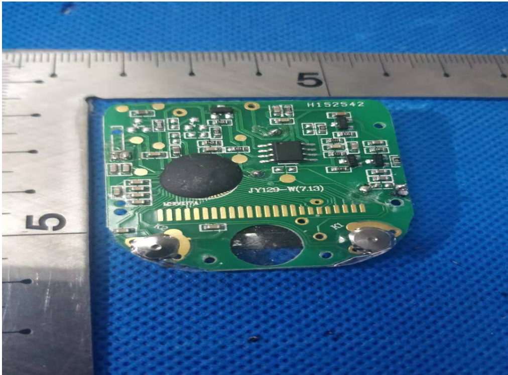
1 EUT Photo (computer)
