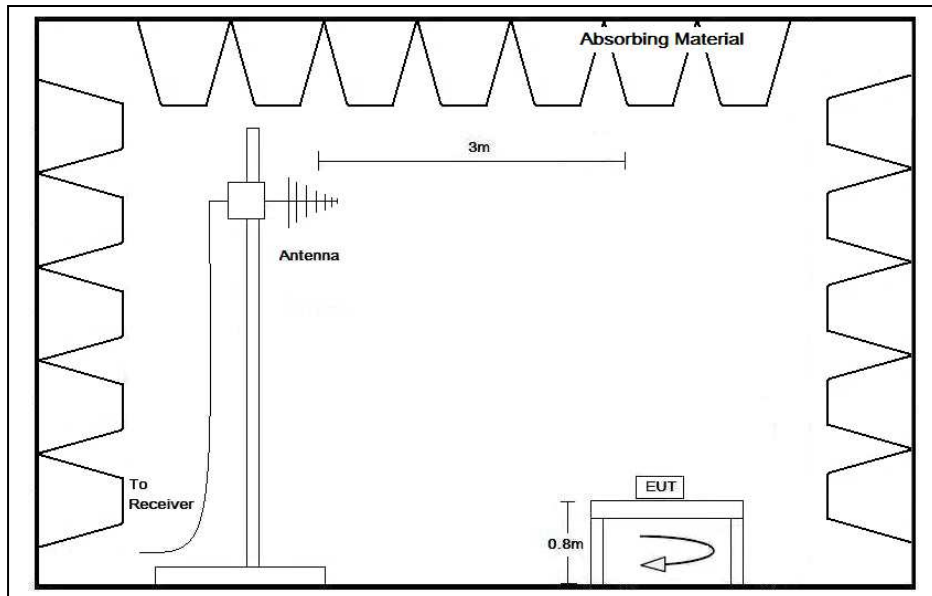
30MHz – 1GHz
