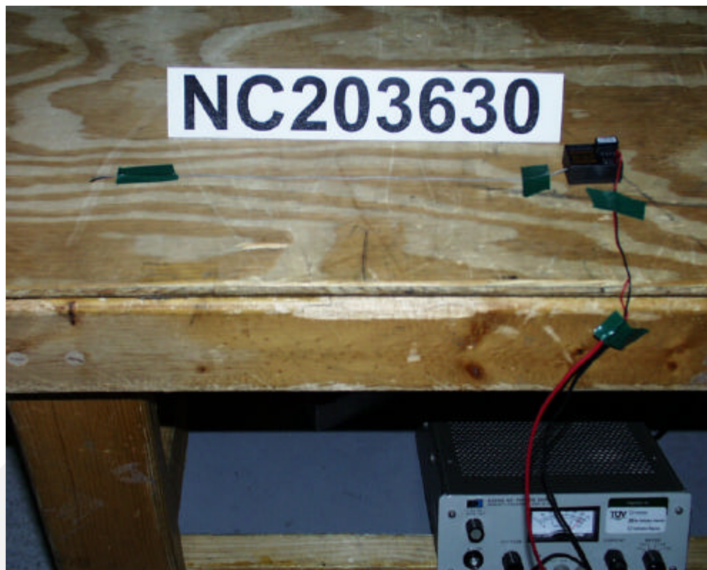
Test-setup photo(s): Radiated emission 30 MHz - 1000 MHz
