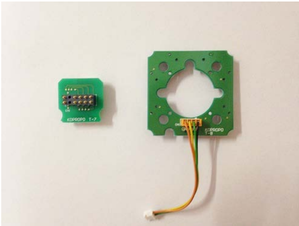
[STERRING UNIT CONNECTOR PCB & SWITCH PCB TOP VIEW]
