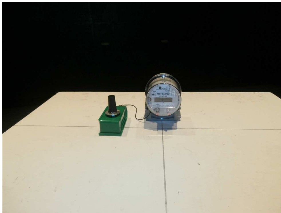
Figure 11: Radiated Emissions - 12S Meter Form External Antenna
