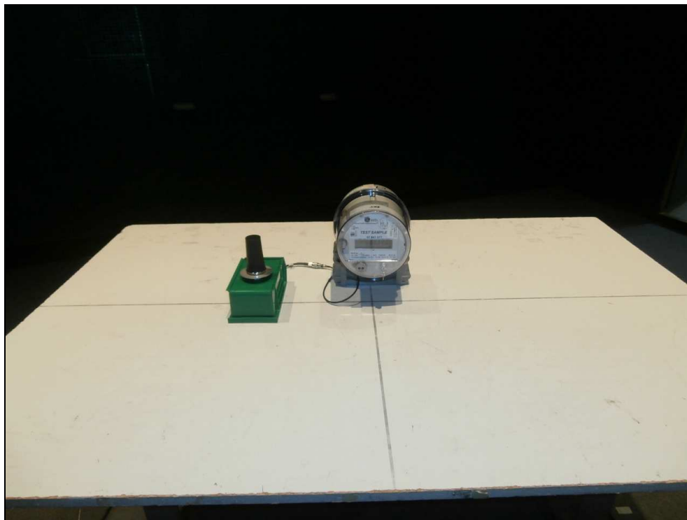
Figure 15: Radiated Emissions - 16S Meter Form External Antenna
