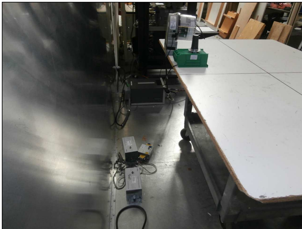
Figure 20: Conducted Emissions – 2S Meter Form
