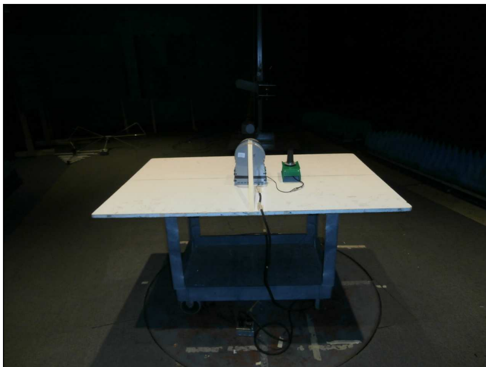
Figure 12: Radiated Emissions - 12S Meter Form External Antenna
