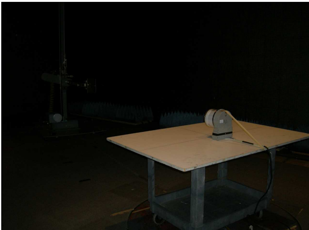
Figure 14: Radiated Emissions – 16S Meter Form Internal Antenna
