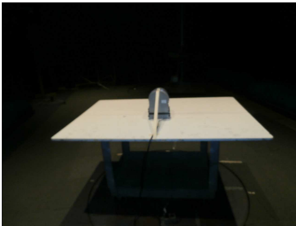
Figure 8: Radiated Emissions – 9S Meter Form Internal Antenna
