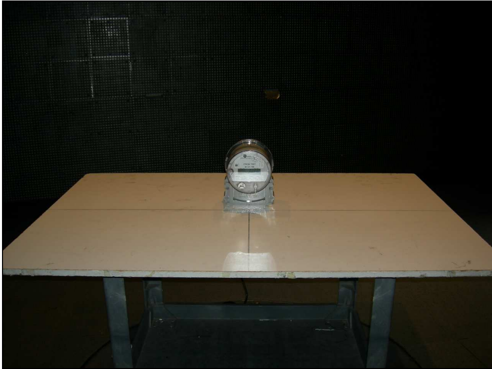
Figure 5: Radiated Emissions – 4S Meter Form Internal Antenna
