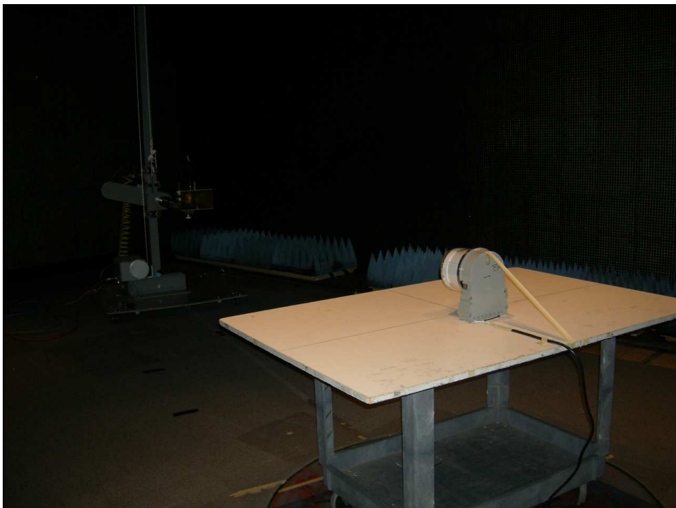
Figure 6: Radiated Emissions – 4S Meter Form Internal Antenna
