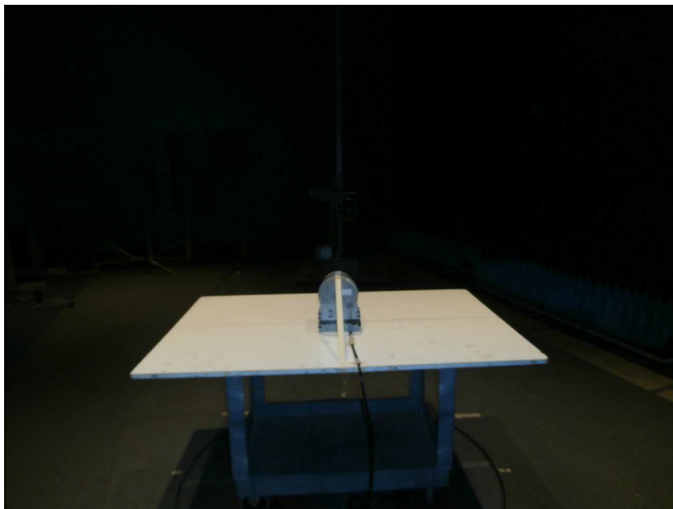
Figure 2: Radiated Emissions – 2S Meter Form Internal Antenna
