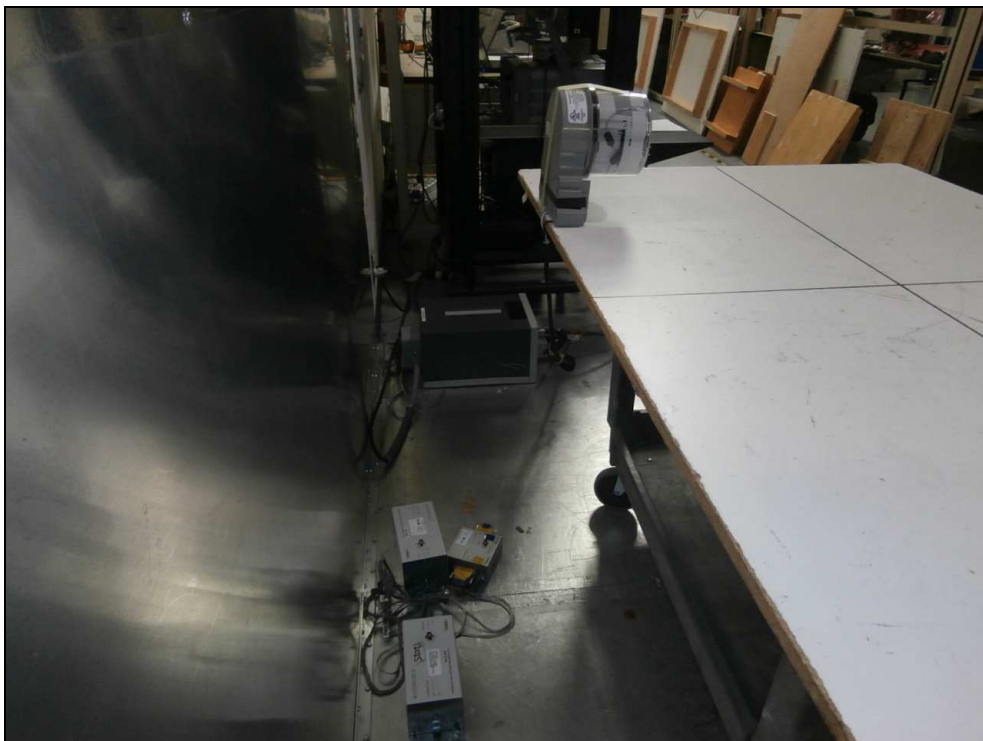
Figure 30: Conducted Emissions – 16S Meter Form
