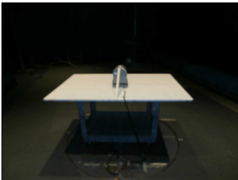
Figure 10: Radiated Emissions – 12S Meter Form Internal Antenna
