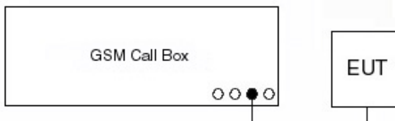
Figure 6-1. GSM/GPRS Conducted Power Test Setup Diagram
