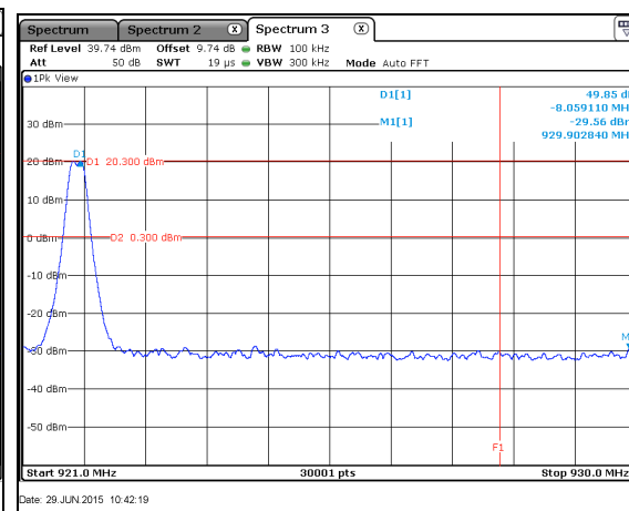
Figure 7.5.1.2-2: Upper Band-edge
